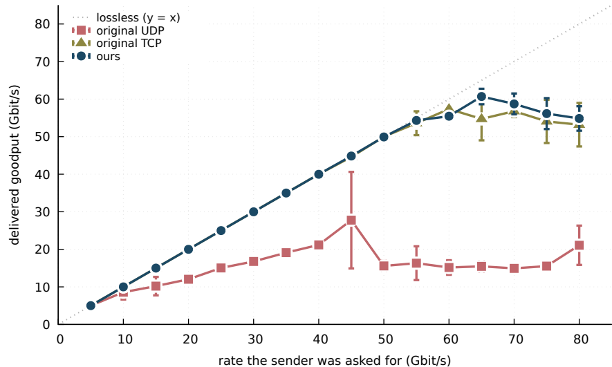
MTU 9000, single flow, one core
