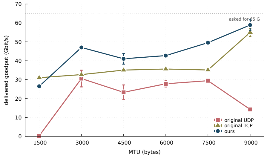
single flow, one core, sender asked for 65 Gbit/s
