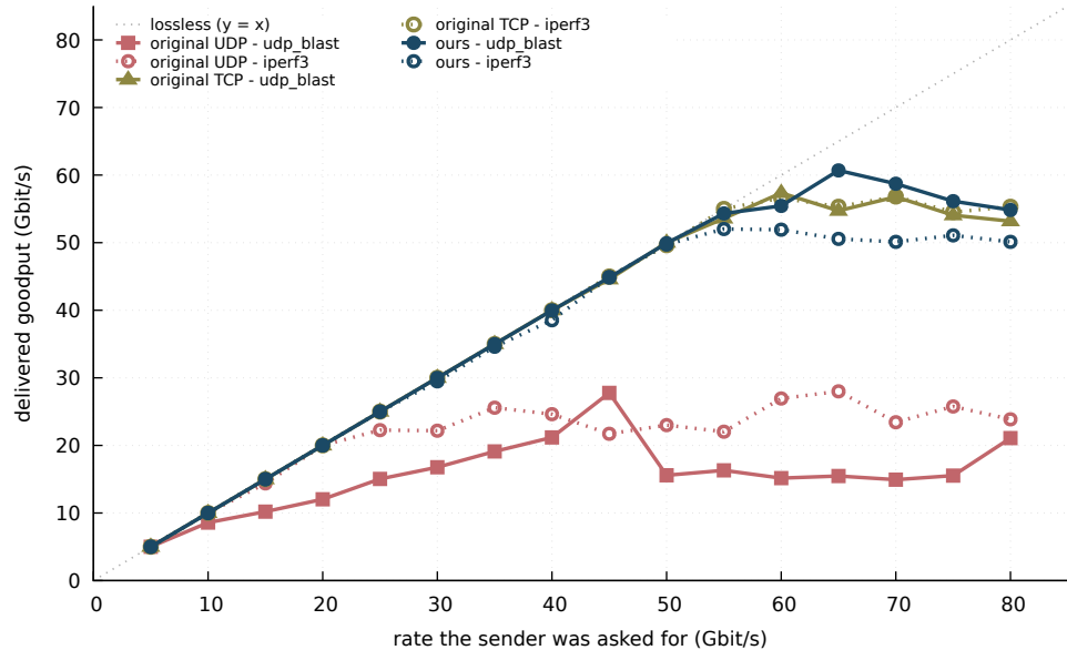
MTU 9000, single flow: does the benchmark tool change the answer?
