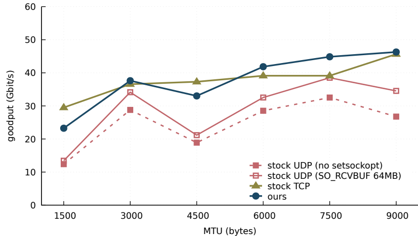
throughput vs MTU (mean over 1/2/4/8/16 flows)
