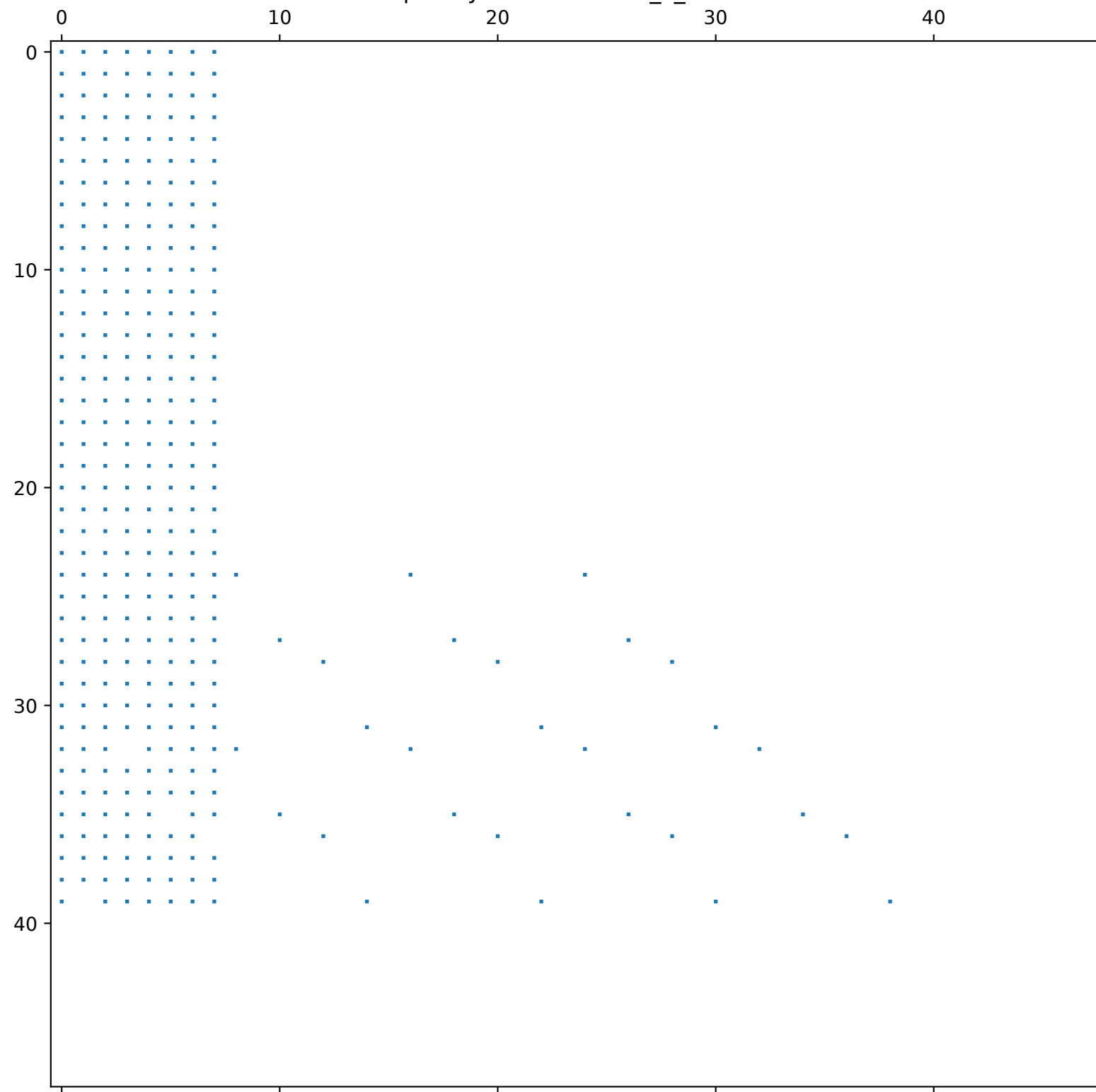
Sparsity Pattern of Nuc_F_matrix
