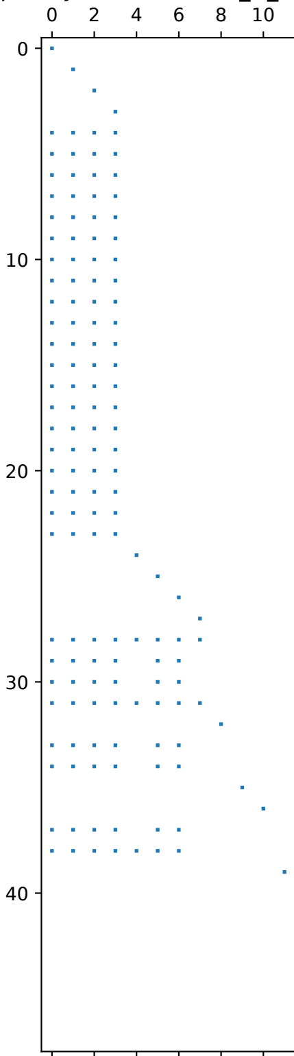
Sparsity Pattern of Nuc_D_matrix
