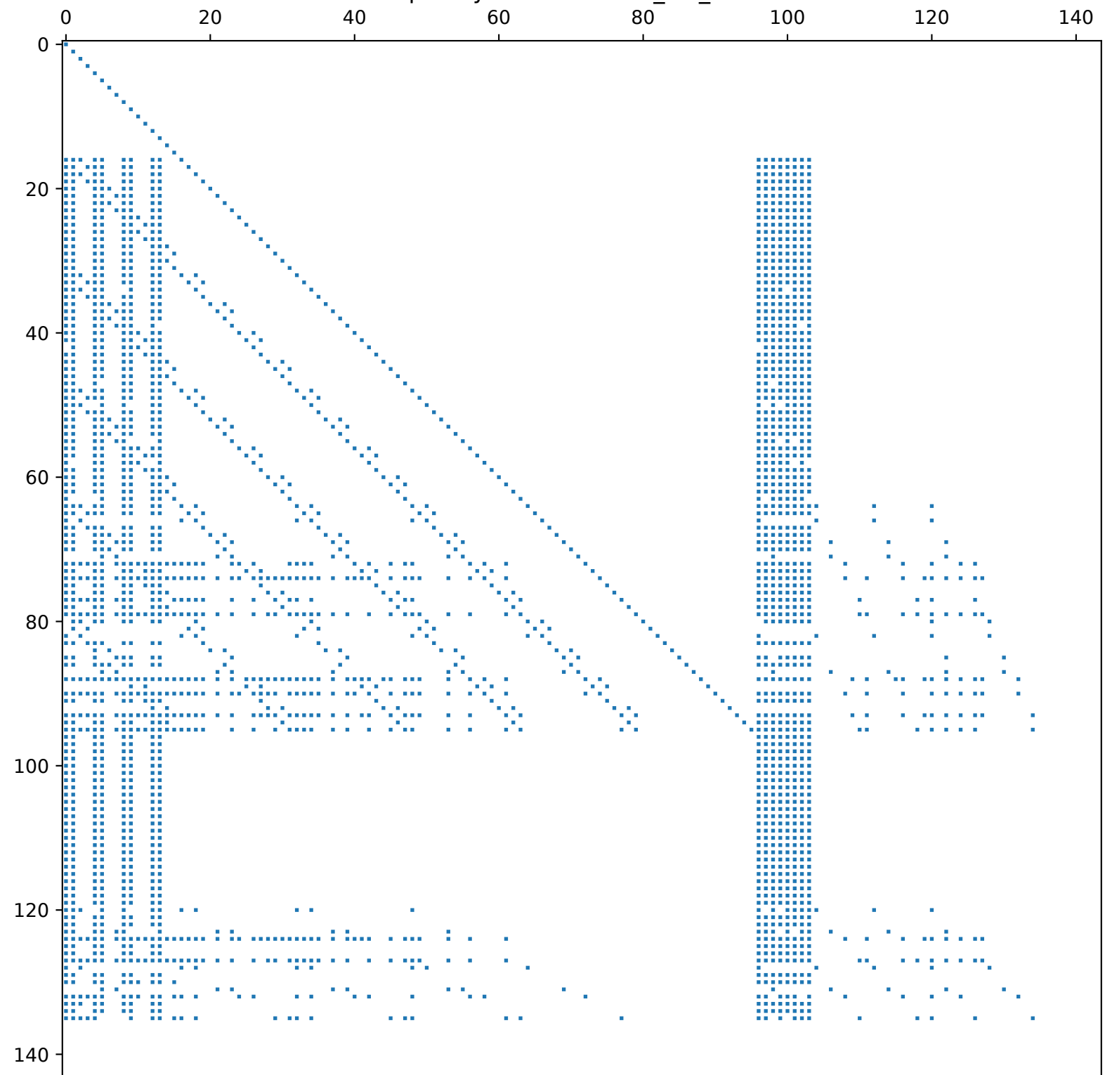
Sparsity Pattern of Nuc_Phi_trunc
