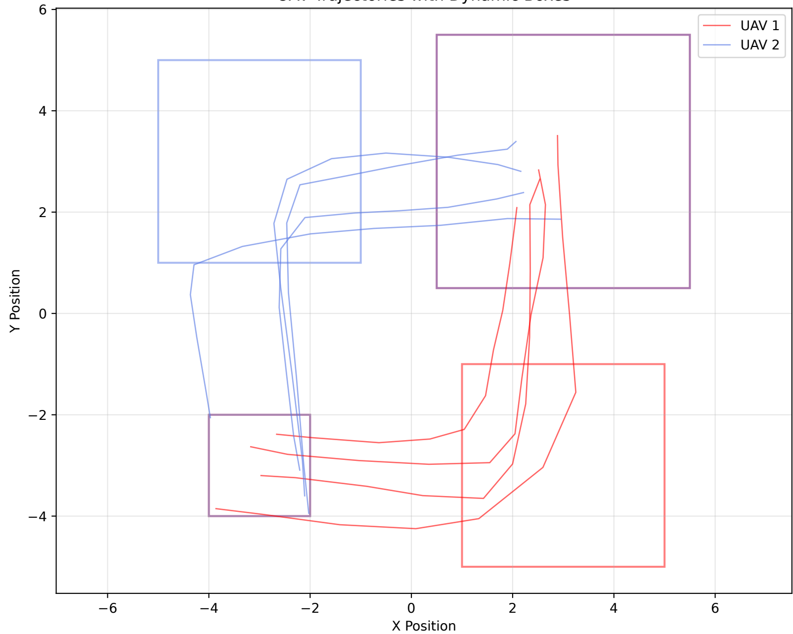
UAV Trajectories with Dynamic Boxes
