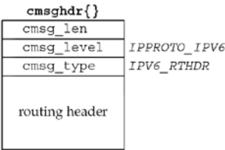
Figure 27.12. Ancillary data object for IPv6 routing header.
