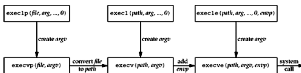
Figure 4.12. Relationship among the six exec functions.
