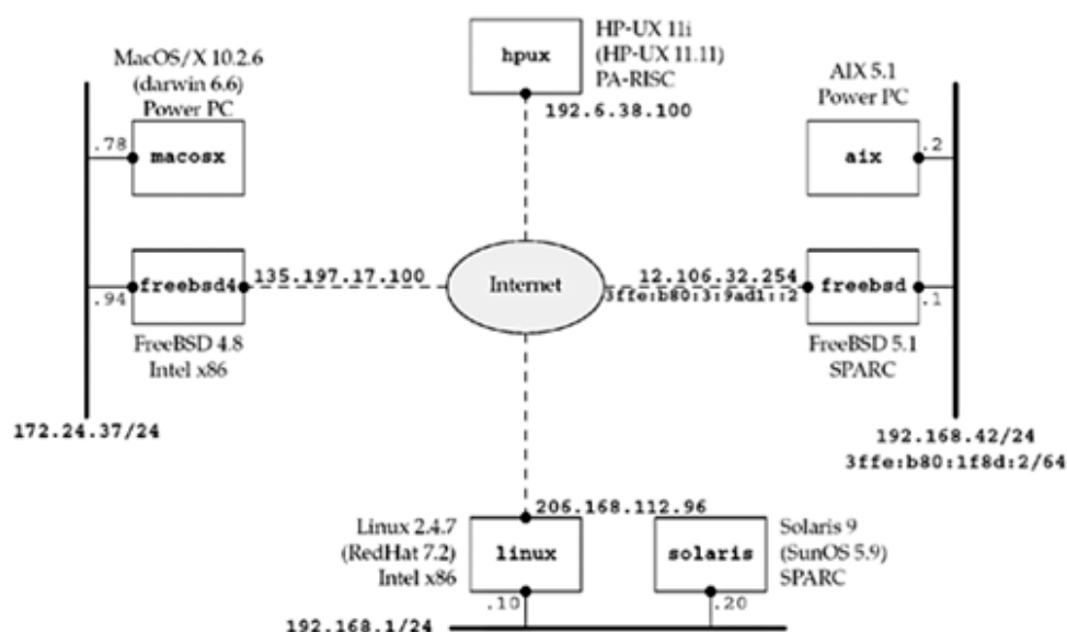
Figure 1.16. Networks and hosts used for most examples in the book
