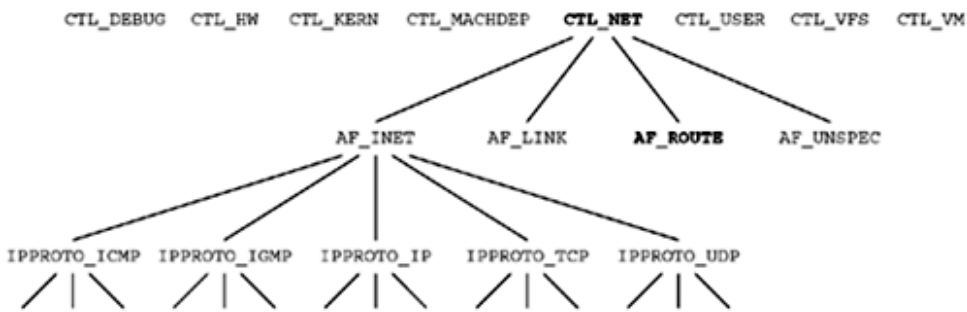
Figure 18.11. Hierarchical arrangement of sysctl names.
