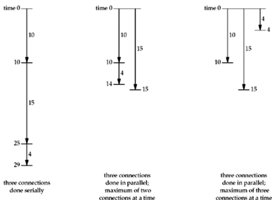
Figure 16.12. Establishing multiple connections in parallel.
