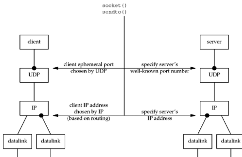
Figure 8.11. Summary of UDP client /server from client's perspective.
