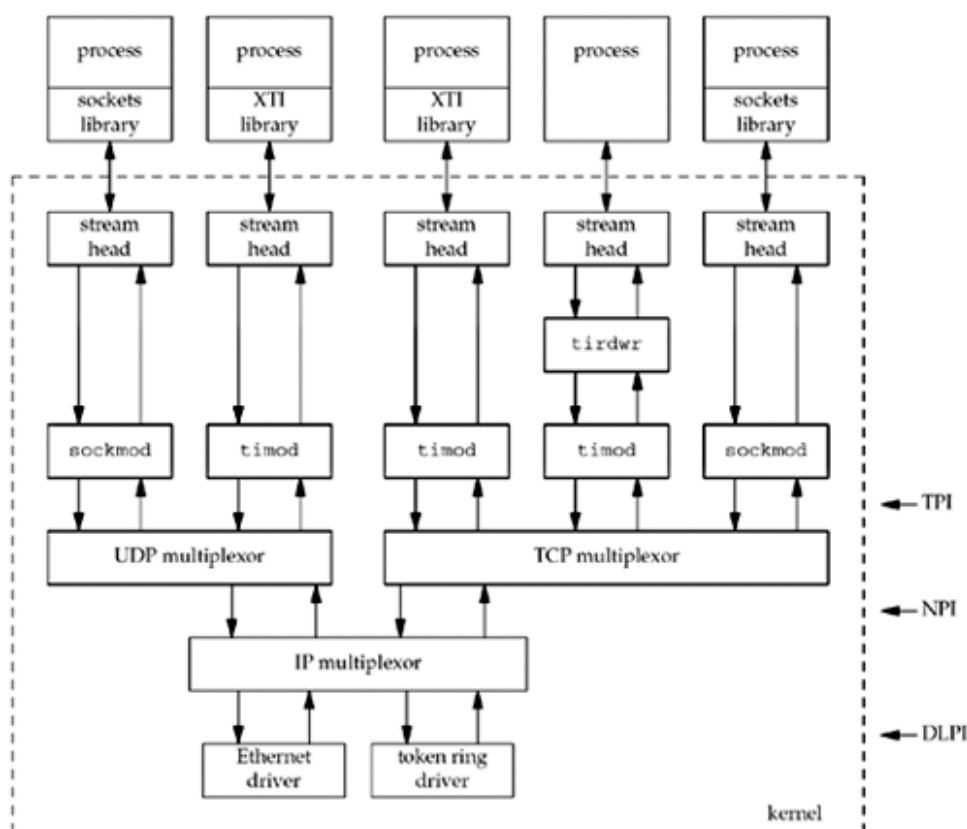
Figure 31.3. A potential implementation of TCP / IP using STREAMS.
