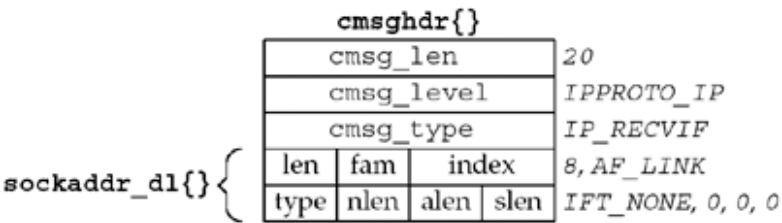
Figure 22.3. Ancillary data object returned for IP_RECVIF .
