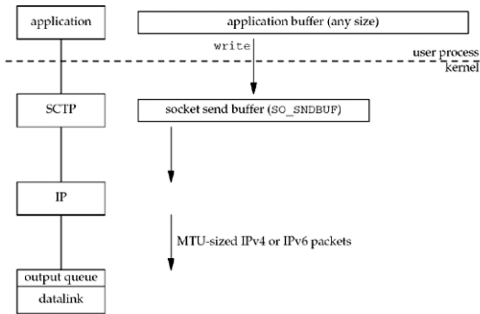
Figure 2.17. Steps and buffers involved when an application writes to an SCTP socket.
