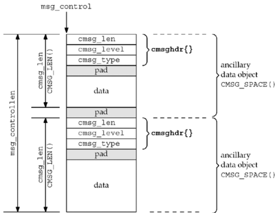
Figure 14.12. Ancillary data containing two ancillary data objects.
