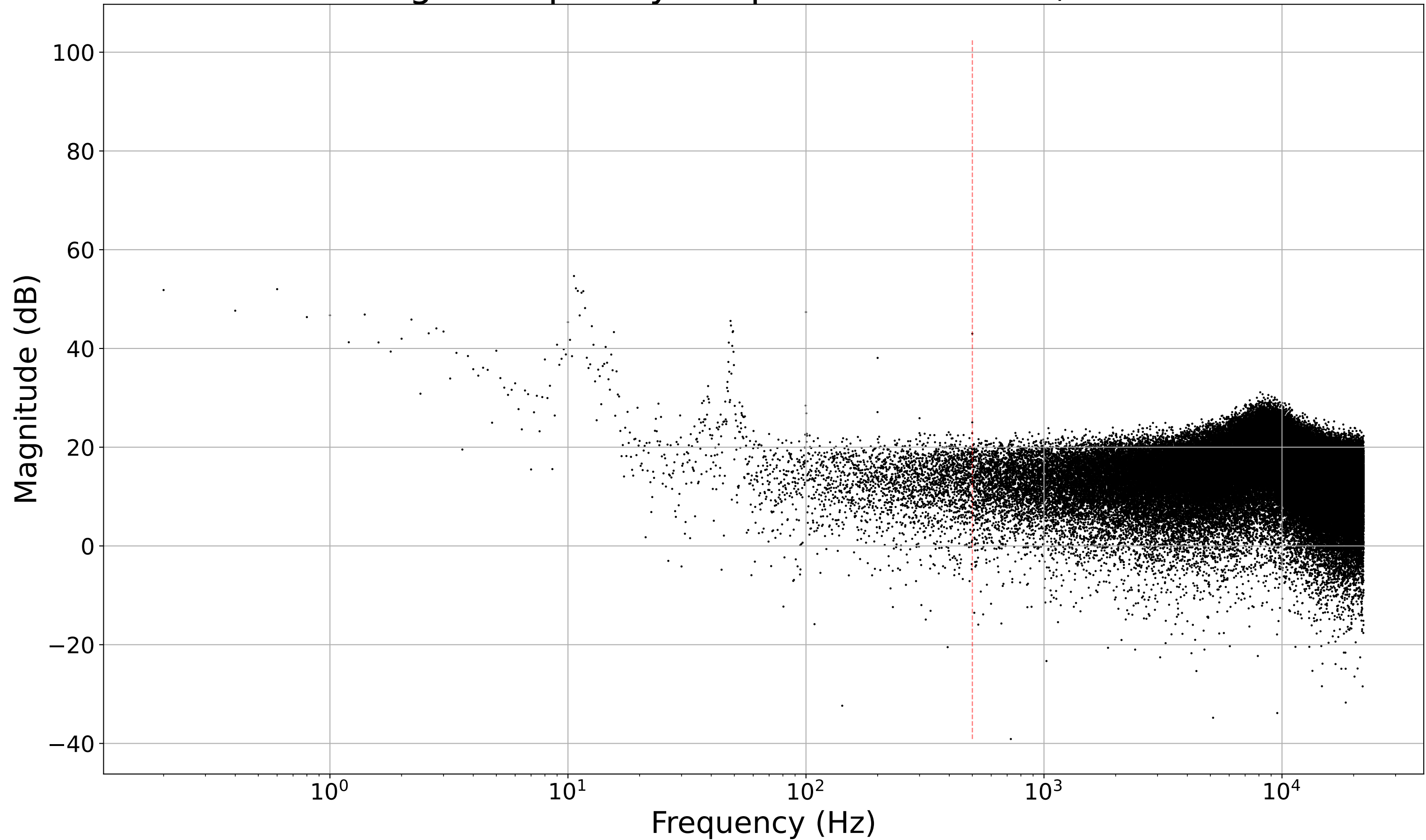
Single Frequency Response at 500 Hz, 0.3 V
