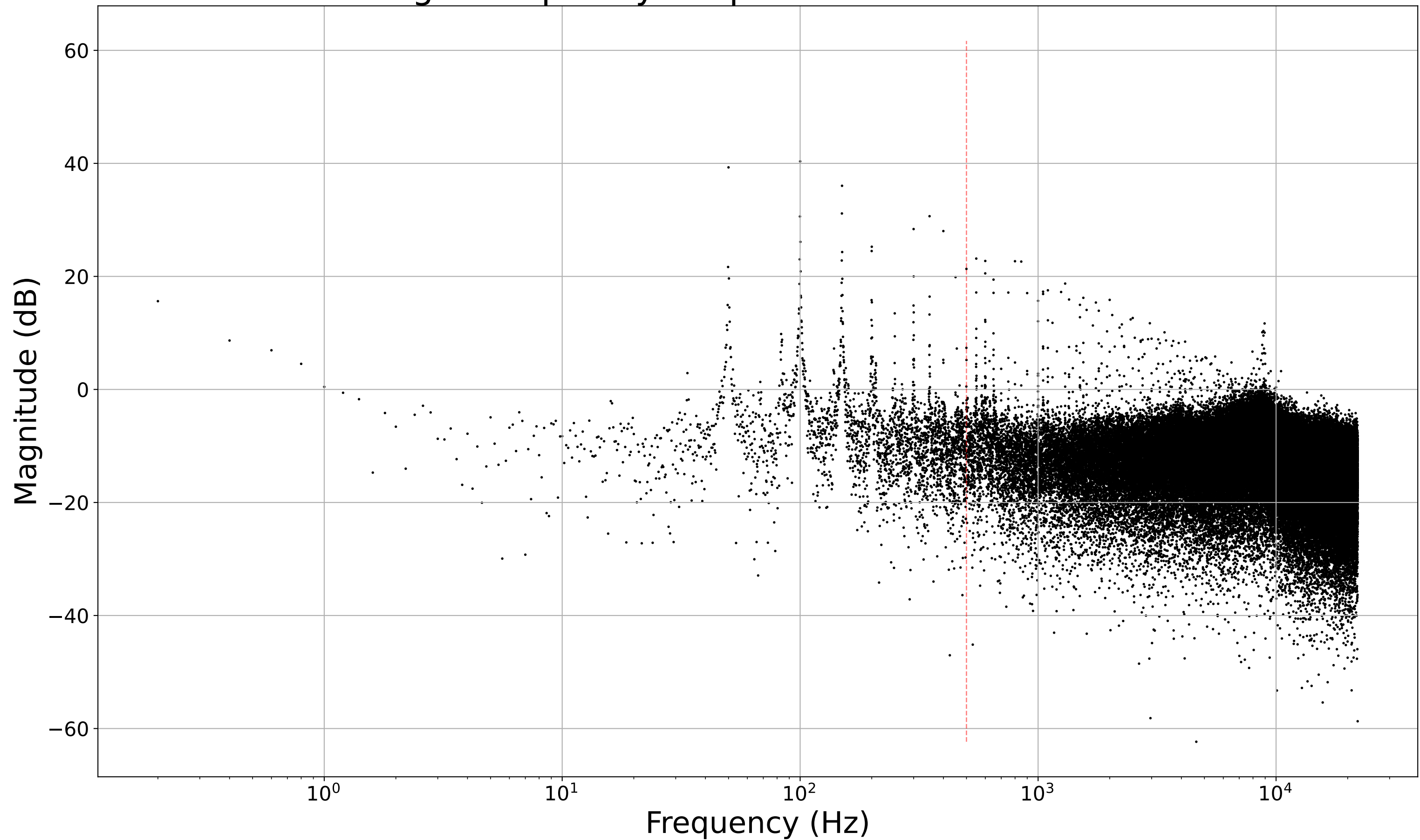
Single Frequency Response at 500 Hz and 3 V
