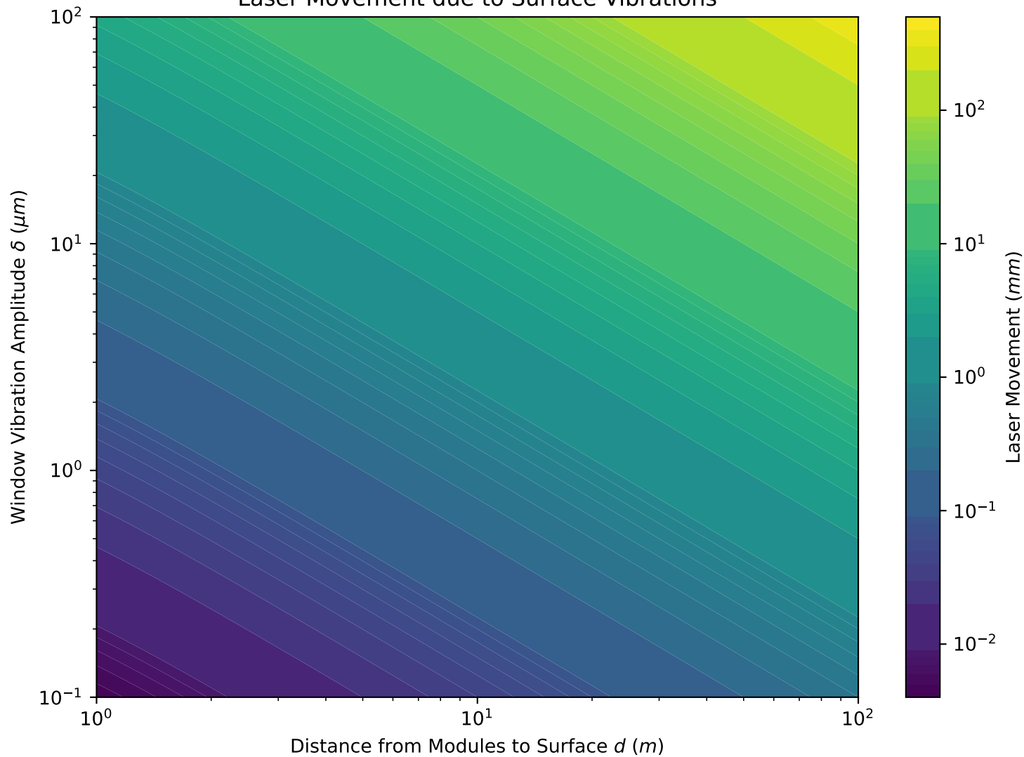
Laser Movement due to Surface Vibrations
