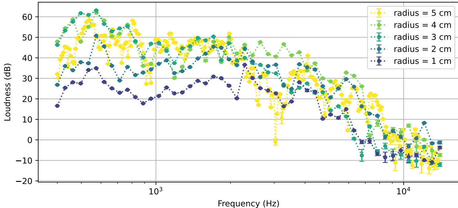
Transfer Function Measurements at Various Drum Sizes
