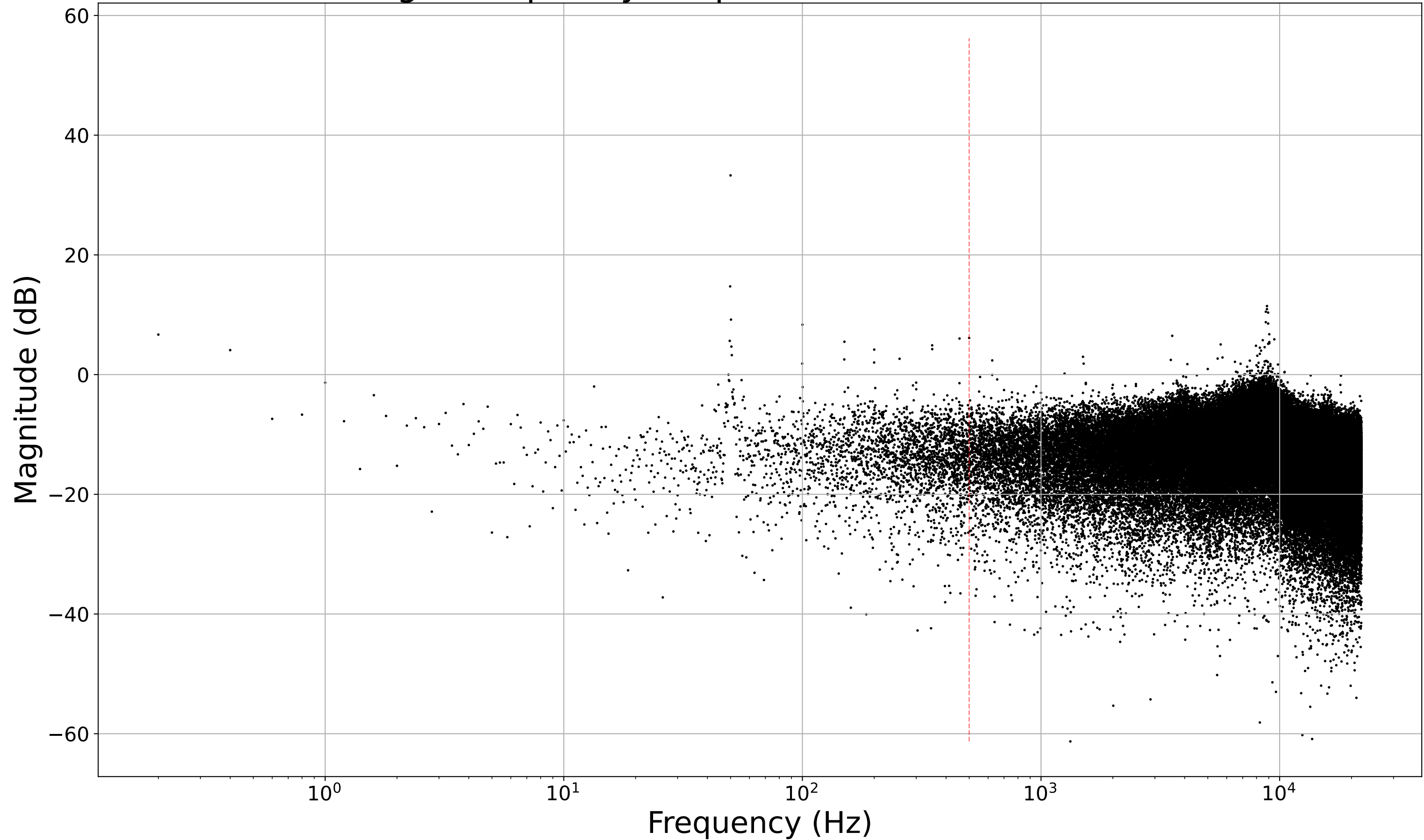
Single Frequency Response at 500 Hz and 0.3 V
