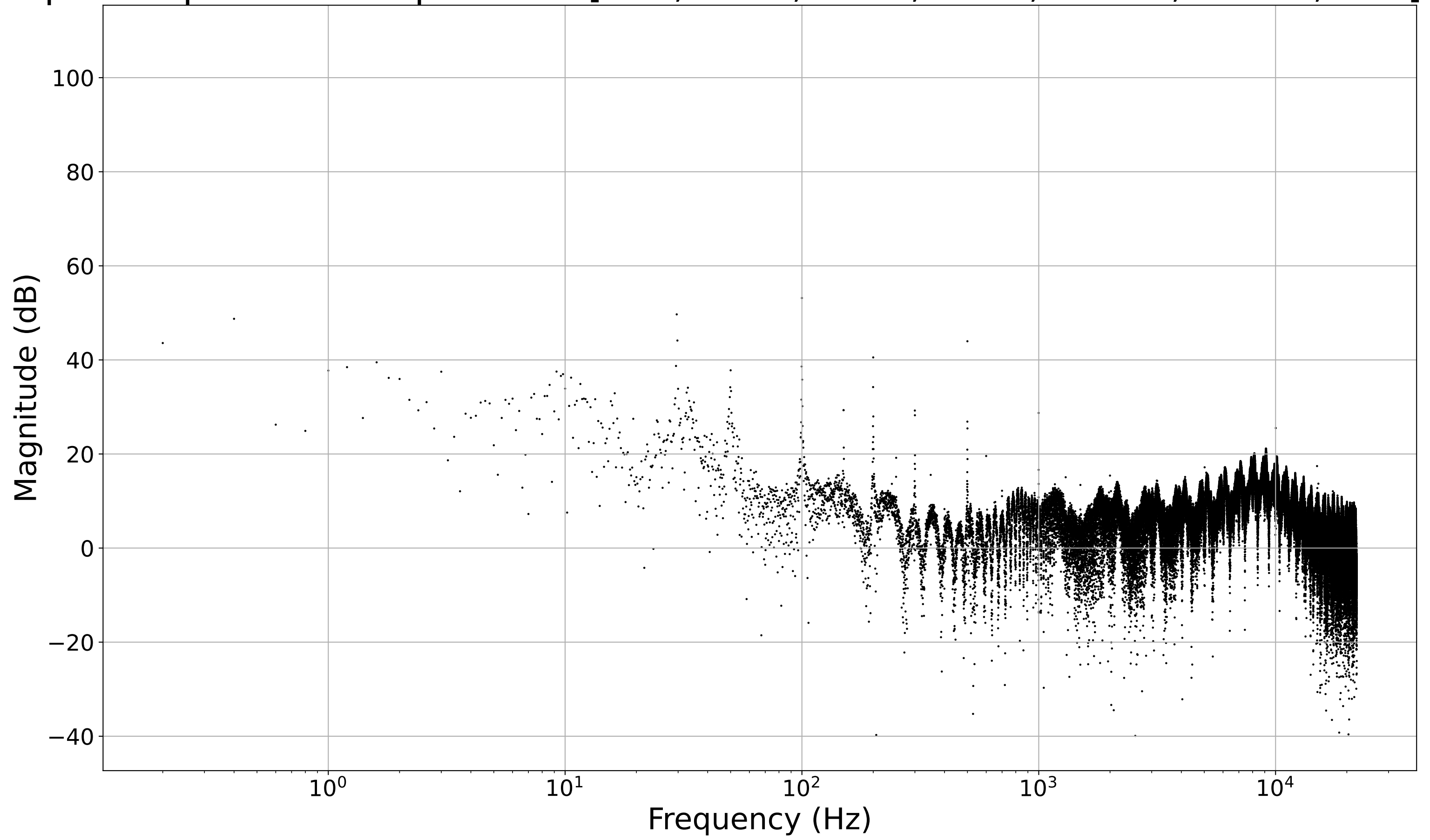
Multiple Frequencies Response at [500, 1000, 2000, 5000, 10000, 15000, 300]
