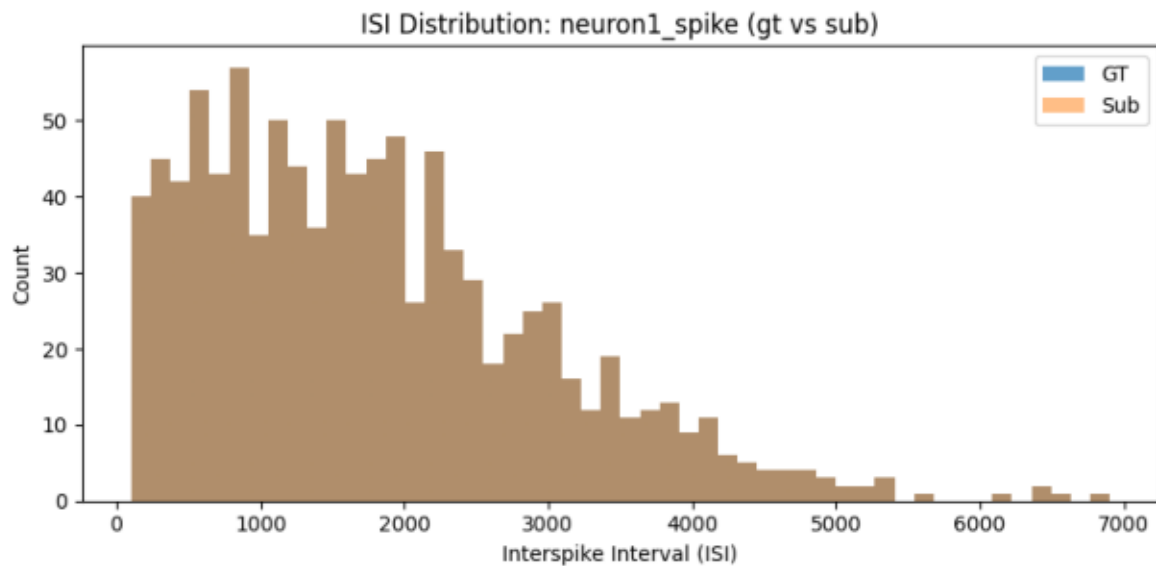
isi_dist_neuron1.png
