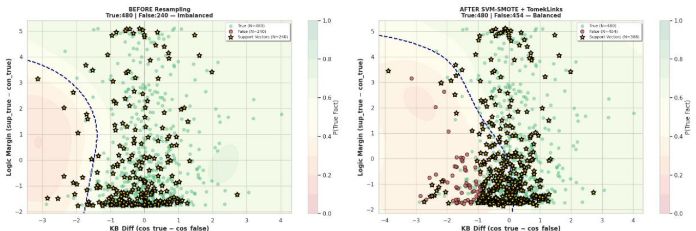
SVM Decision Boundary — Before vs After Resampling
