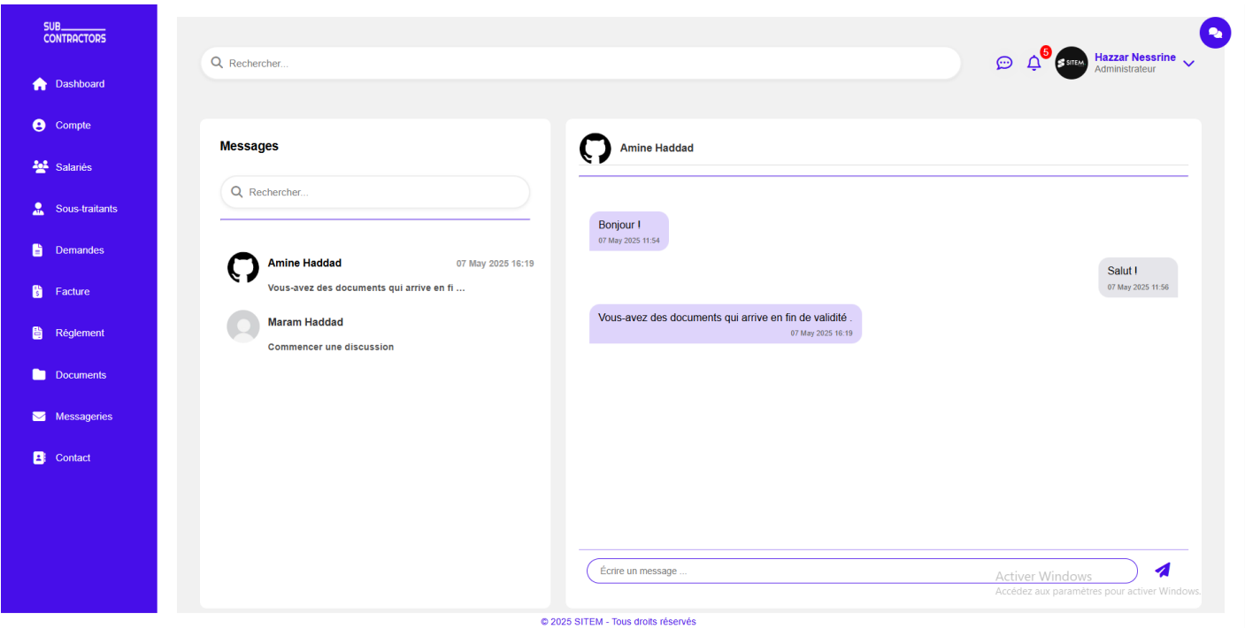
FIGURE 4.11 – Interface Messagerie
