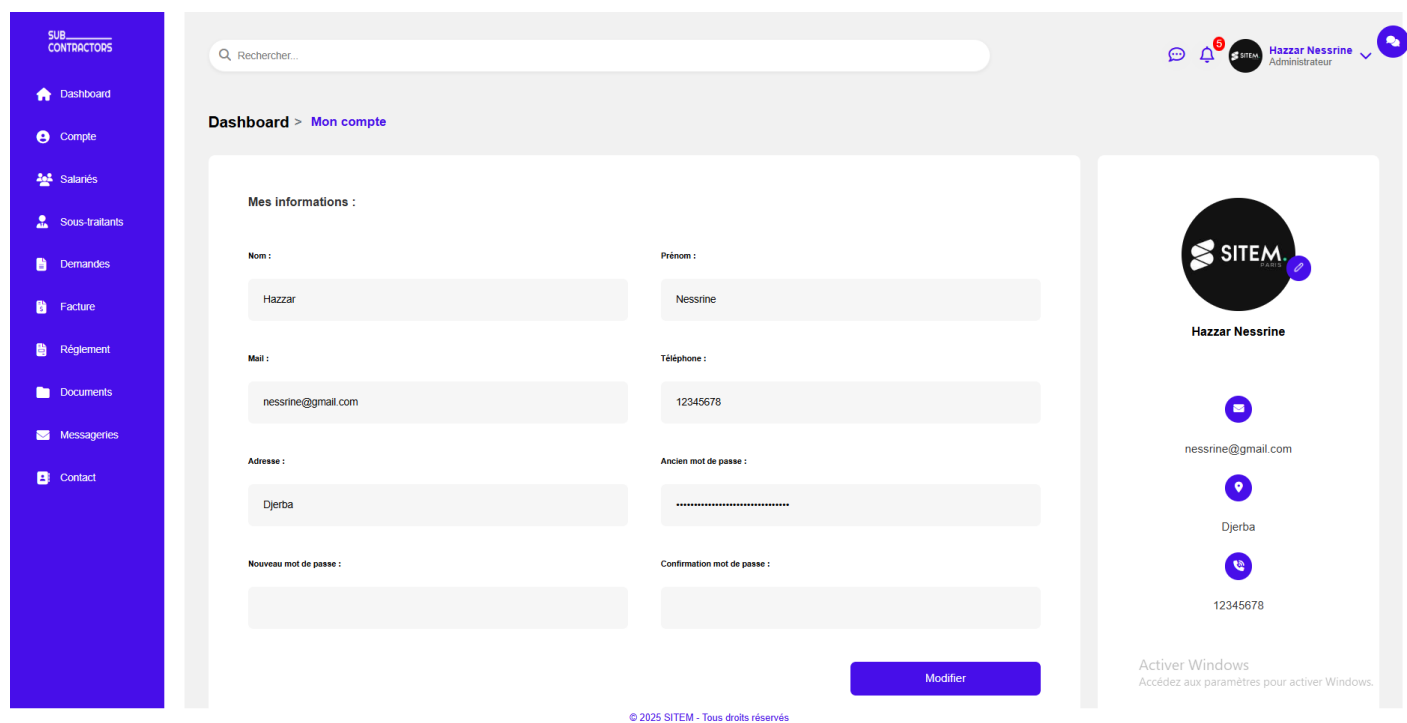
FIGURE 4.3 – Interface Profile
