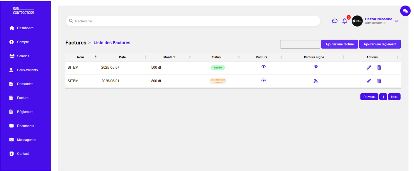
FIGURE 4.10 – Interface Facture
