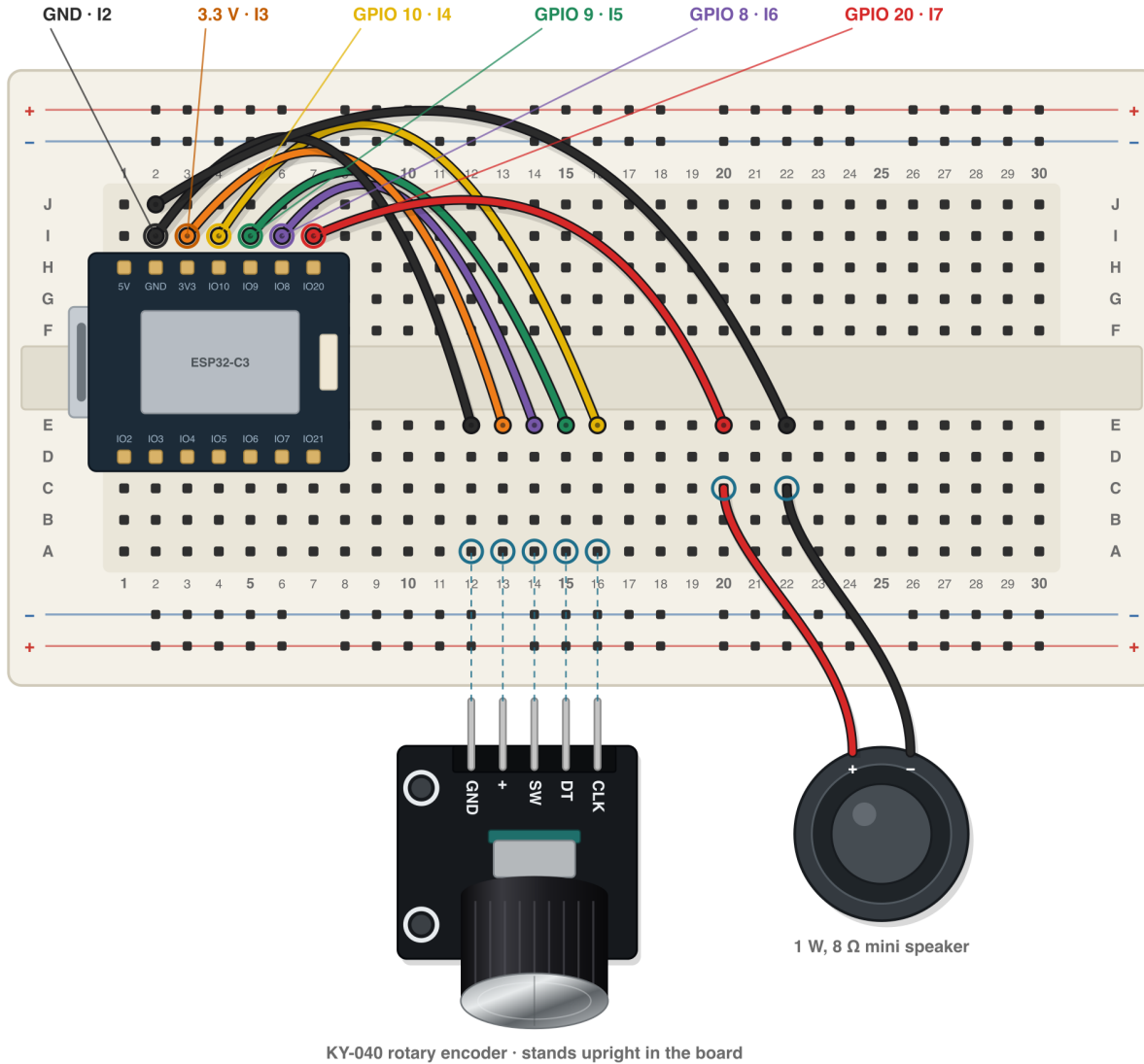
Figure 7.1: Encoder and speaker wired to the XIAO ESP32-C3
