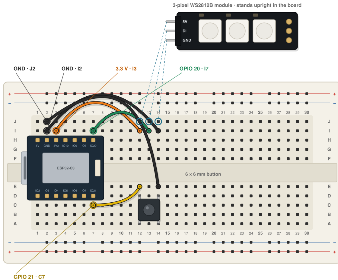
Figure 5.1: Connect the LED strip and button to the XIAO ESP32-C3.
