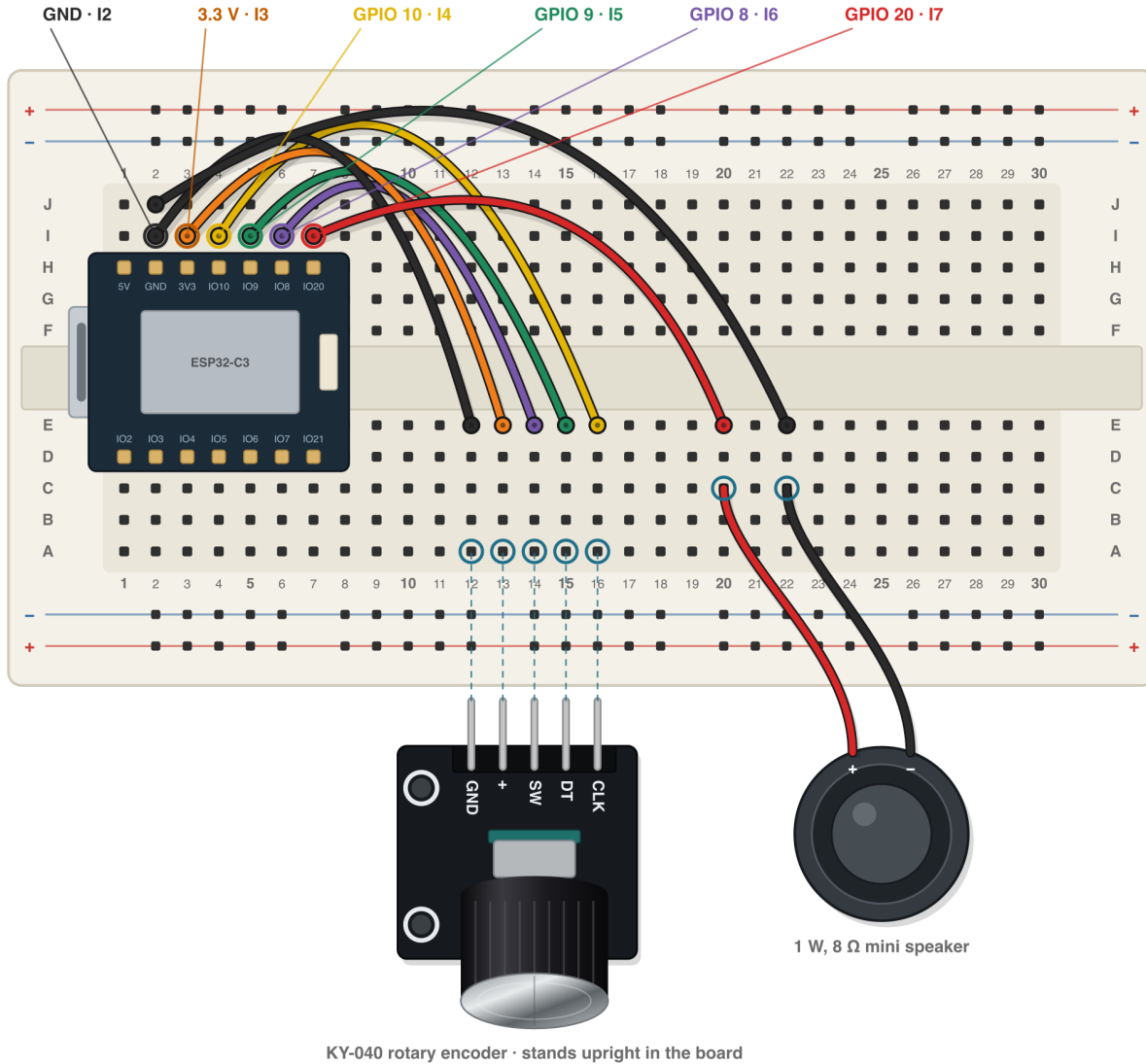
Figure 6.1: Encoder and speaker wired to the XIAO ESP32-C3
