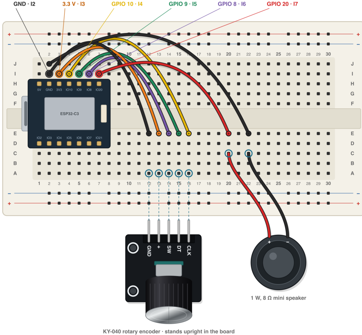
Figure 6.1: Encoder and speaker wired to the XIAO ESP32-C3
