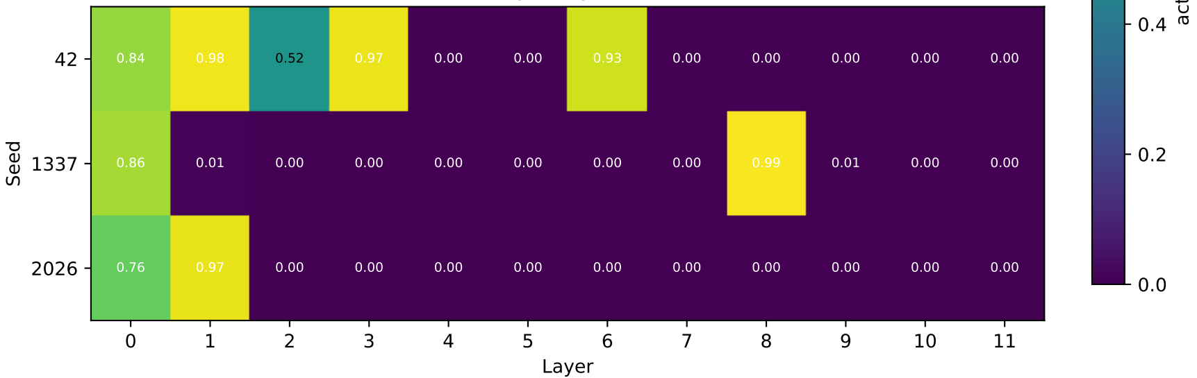
v4-rwkv7-nsa: per-layer active fraction
