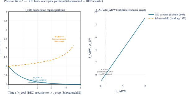
FIG. 1. Opposite signs of dT_H/dt under evaporation. The Schwarzschild branch (amber, dashed) heats and terminates in finite time, while the sonic branch (blue, solid) cools and reaches zero temperature only asymptotically; the right panel shows the substrate response \delta_{\text{ADW}} = (\alpha_{\text{ADW}} - 1)\Lambda_{\text{UV}} vanishing at the bare induced limit \alpha_{\text{ADW}} = 1 . The critical mass separating the branches is Eq. (1), equivalently Eq. (2). Formal witnesses: T_H_schwarzschild_strict_decreasing and T_H_acoustic_evolution_strict_decreasing , combined by regime_partition_criterion .
