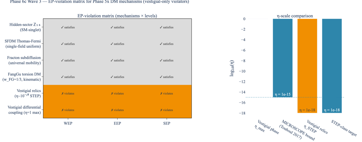
FIG. 1. Equivalence-principle violation matrix (left) and \eta -scale comparison (right). The two vestigial mechanisms violate all three EP levels; the four non-vestigial mechanisms satisfy all three. The right panel locates the vestigial-phase \eta_{\max} = 1 , the MICROSCOPE bound \eta < 10^{-15} [2], the vestigial-relic \eta \sim 10^{-18} , and the next-generation satellite-test target \eta \sim 10^{-18} on a common log scale.
