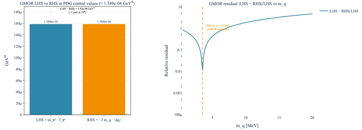
FIG. 1. Gell-Mann–Oakes–Renner relation at PDG/FLAG central values. Left: side-by-side bars at LHS \approx 1.589 \times 10^{-4} \text{ GeV}^4 and RHS \approx 1.589 \times 10^{-4} \text{ GeV}^4 , visually indistinguishable, confirming the relation holds to \sim one part in 10^4 (residual \sim 4 \times 10^{-8} \text{ GeV}^4 ). Right: relative residual |LHS - RHS|/LHS as the input quark mass m_q is swept; the minimum at m_q \approx 3.5 \text{ MeV} (PDG average u/d quark mass [4]) confirms the consistent point. Sources: [2–4].
