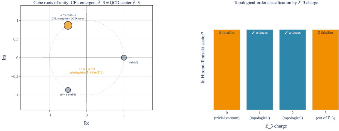
FIG. 1. CFL emergent \mathbb{Z}_3 identifies with QCD center \mathbb{Z}_3 . Left: cube roots of unity \{1, \omega, \omega^2\} on the complex unit circle. The CFL emergent generator (defined independently from the diquark-sector one-form symmetry per [4]) and the QCD center generator (from the bare-gauge center symmetry per [7] and the companion module) coincide at the same point \omega = \exp(2\pi i/3) . The sum 1 + \omega + \omega^2 = 0 is the algebraic fingerprint distinguishing \mathbb{Z}_3 from \mathbb{Z}_2 . Right: \mathbb{Z}_3 charge classification across the three sectors \{0, 1, 2\} plus the out-of- \mathbb{Z}_3 value c = 3 falsifier; the topologically ordered sectors (charges 1, 2) are the structural witness for [4]’s topological-order-beyond-Landau–Ginzburg framing.
