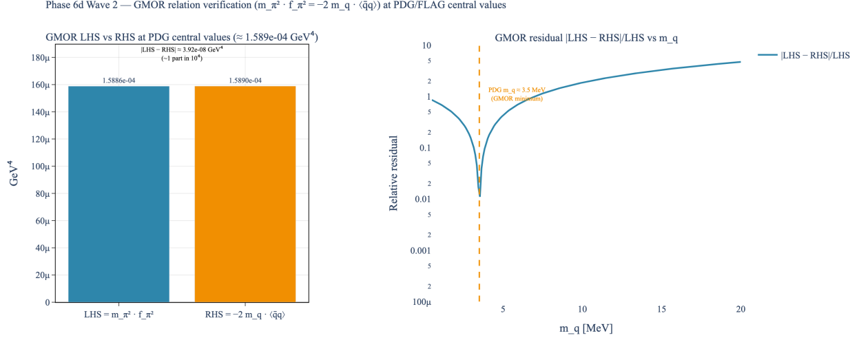
FIG. 1. Gell-Mann–Oakes–Renner relation at PDG/FLAG central values. Left: side-by-side bars at LHS \approx 1.589 \times 10^{-4} \text{ GeV}^4 and RHS \approx 1.589 \times 10^{-4} \text{ GeV}^4 , visually indistinguishable, confirming the relation holds to \sim one part in 10^4 (residual \sim 4 \times 10^{-8} \text{ GeV}^4 ). Right: relative residual |LHS - RHS|/LHS as the input quark mass m_q is swept; the minimum at m_q \approx 3.5 \text{ MeV} (PDG average u/d quark mass [4]) confirms the consistent point. Sources: [2–4].
