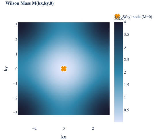
FIG. 2. Wilson mass M(k_x, k_y, 0) on the k_z = 0 plane of the Brillouin zone. The unique zero at (0, 0) marks the Weyl node. All other points have M > 0 .
