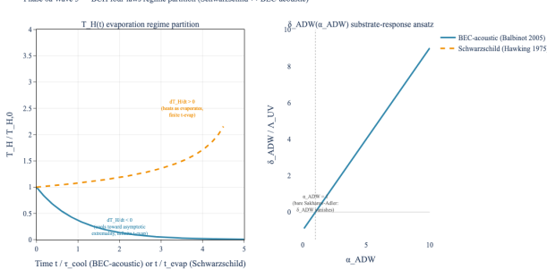
FIG. 1. Headline result. Sign-flip of dT_H/dt between the Schwarzschild (amber dashed; Hawking 1975 [1]; dT_H/dt > 0 , finite t_{\text{evap}} ) and BEC-acoustic (steel-blue solid; Balbinot et al. [2]; dT_H/dt < 0 , asymptotic extremality at infinite time) regimes during Hawking-radiation evaporation. Left panel: T_H(t) contrast. Right panel: substrate-response coefficient \delta_{ADW} = (\alpha_{ADW} - 1)\Lambda_{UV} vanishing at \alpha_{ADW} = 1 . The critical mass M_c separating regimes is given by Eq. (3). Lean witness: T_H_acoustic_evolution_strict_decreasing + T_H_schwarzschild_strict_decreasing .
