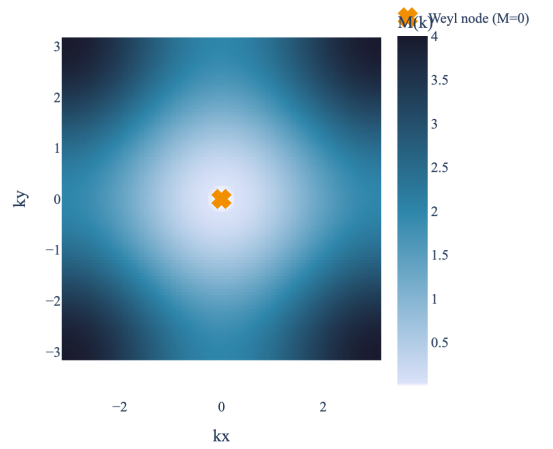
Wilson Mass M(k_x, k_y, 0)
