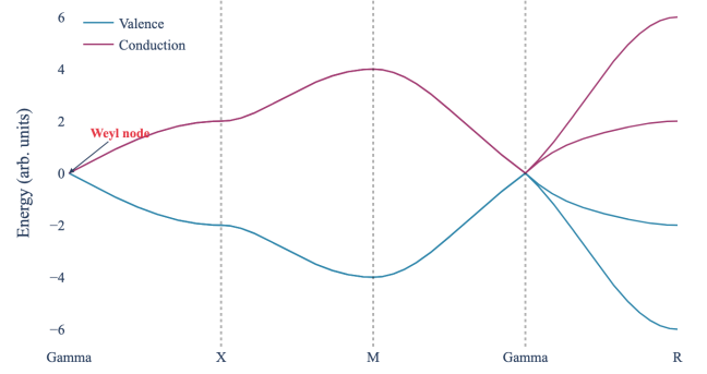
GT BdG Band Structure ( r=1 )
