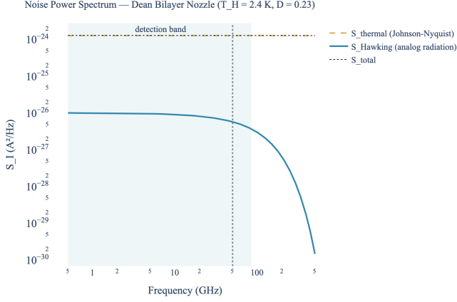
FIG. 2. Current noise power spectral density for the Dean bilayer nozzle (realistic greybody \Gamma_0 \approx 0.9994 per Eq. (??)). \Delta S_I (blue) sits \sim 2 orders below the Johnson-Nyquist background S_{\text{thermal}} (amber dashed). The Hawking signal is flat below \omega_H \approx 51 GHz and Boltzmann-suppressed above. Shaded region: detection band (0.5 GHz to 85 GHz).
