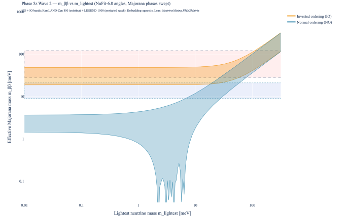
FIG. 2. Effective Majorana mass m_{\beta\beta} against the lightest neutrino mass m_{\text{lightest}} . Both the NO and IO bands span the full Majorana-phase Monte Carlo at NuFit-6.0 [?] best-fit angles. Horizontal bands: KamLAND-Zen 800 [?] current 90% CL bound (28-122 meV; NME spread) and LEGEND-1000 99.7% CL projected discovery reach (9-21 meV) [?]. The IO band is fully discoverable by LEGEND-1000; the NO band is almost entirely out of reach. The result is embedding-agnostic across I/II/III. Lean reference: NeutrinoMixing.PMNSMatrix .
