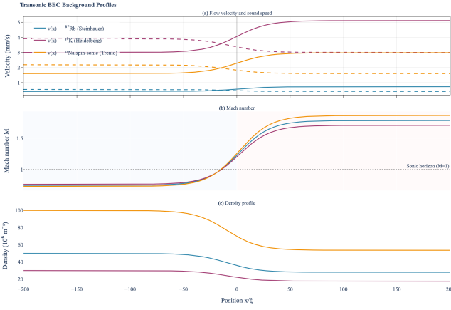
FIG. 1. Transonic background profiles for three BEC analog Hawking experiments: Steinhauer ^{87}\text{Rb} (blue), Heidelberg ^{39}\text{K} (berry), and Trento ^{23}\text{Na} spin-sonic (amber). Panels show velocity and sound speed, Mach number, and density profiles near the sonic horizon.
