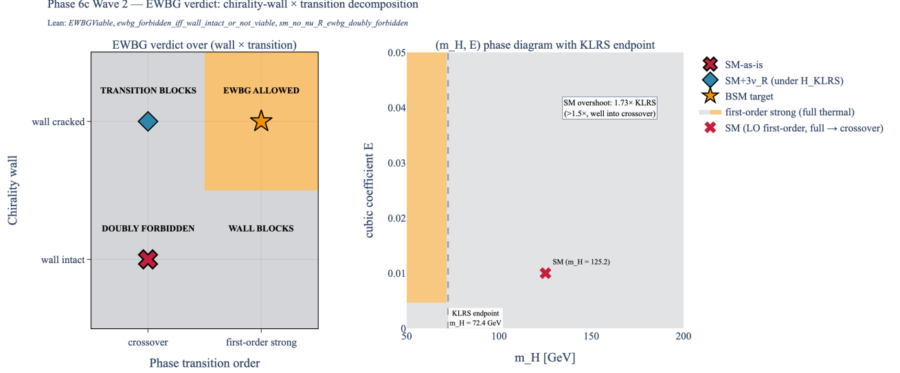
FIG. 1. EWBG verdict over the (chirality wall \times transition order) decomposition. Left: 2 \times 2 outcome matrix. SM-as-is sits at (intact wall + crossover under H_{KLRS} ); doubly forbidden . SM-with- 3\nu_R sits at (cracked wall + crossover); transition-blocked. BSM target (extra scalars producing strong first-order EWPT) sits at (cracked wall + first-order strong); allowed. Right: the (m_H, E) phase diagram with the KLRS / CFH lattice endpoint at m_H = 72.4 GeV. The PDG SM at m_H = 125.20 GeV sits well to the right of the endpoint (overshoot ratio \approx 1.73 > 1.5 ), placing the resummed transition firmly in the crossover region. Lean: ewbg_forbidden_iff_wall_intact_or_not_viable, sm_no_nu_R_ewbg_doubly_forbidden, sm_klrs_overshoot_ratio_gt_threshold .
