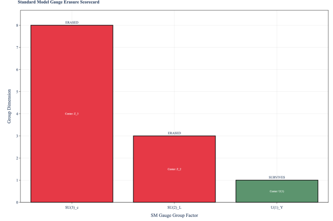
FIG. 1. Standard Model gauge erasure scorecard. SU(3)_c (8 generators) and SU(2)_L (3 generators) are erased by hydrodynamization; only U(1)_Y (1 generator) survives via the 1-form Goldstone mechanism.
