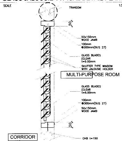
5 GLASS JALOUSIE TYPICAL DETAIL SECTIONS A-5 SCALE 1:5M
