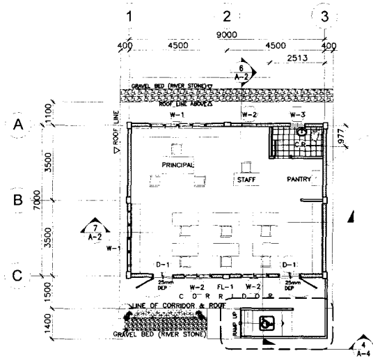
2 PRINCIPAL'S OFFICE & FACULTY ROOM FLOOR PLAN A-2 SCALE 1:100M
