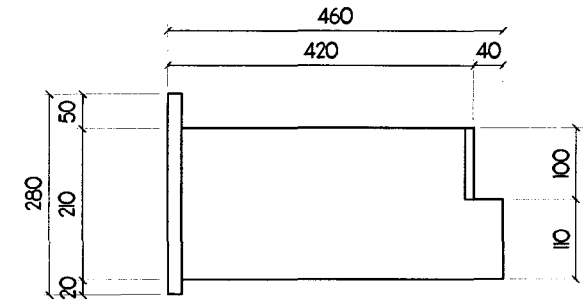
4 RIGHT-SIDE VIEW 10 SCALE 1 : 25 M
