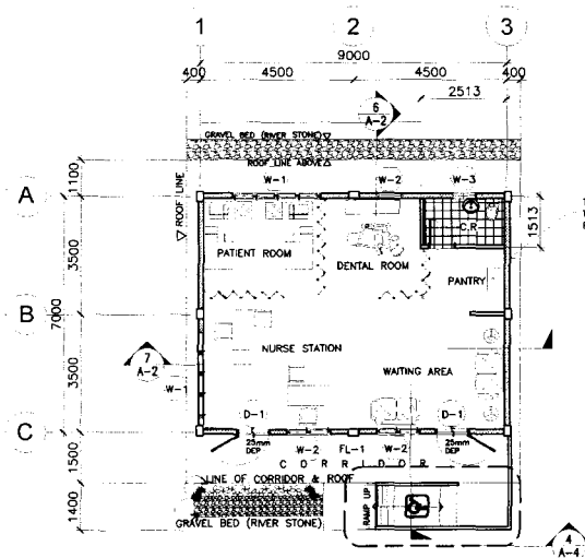
1 SCHOOL CLINIC FLOOR PLAN A-2 SCALE 1:100M
