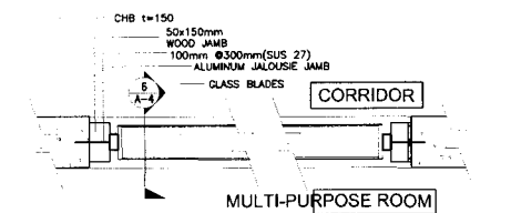
4 GLASS JALOUSIE TYPICAL DETAIL PLANS A-5 SCALE 1:5M
