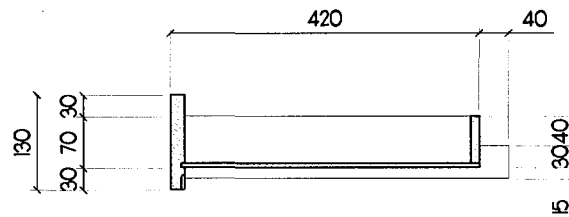
7 SECTION THRU-A 9 SCALE 1 : 25 M
