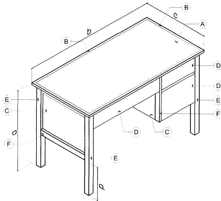
FRONT-LEFT SIDE ISOMETRIC VIEW 1 SCALE 1 : 50 M
