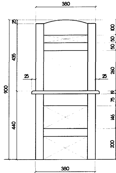
2 FRONT VIEW 2 SCALE 1:25 M
