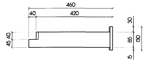
6 LEFT-SIDE VIEW 9 SCALE 1 : 25 M
