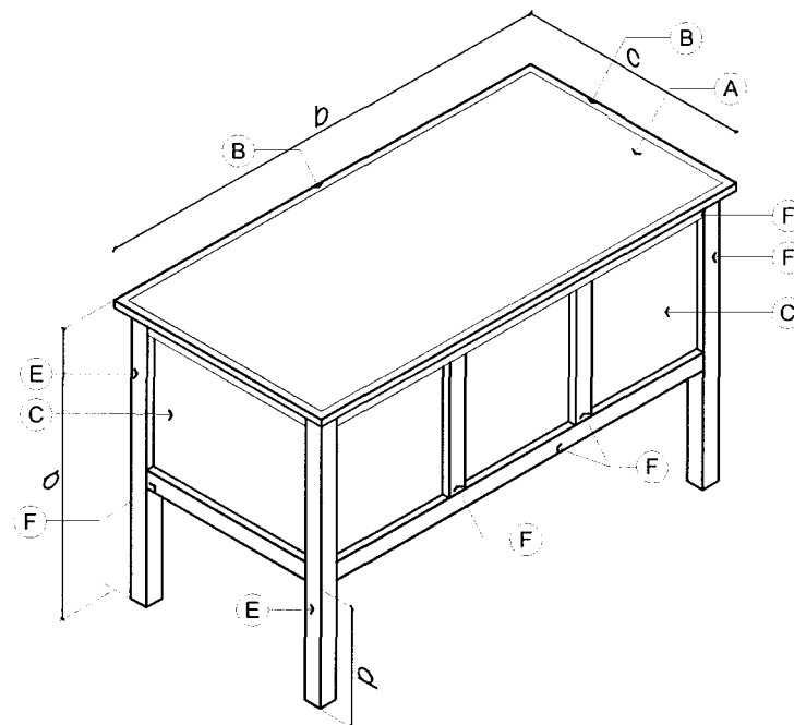
REAR-RIGHT SIDE ISOMETRIC VIEW 2 SCALE 1 : 50 M
