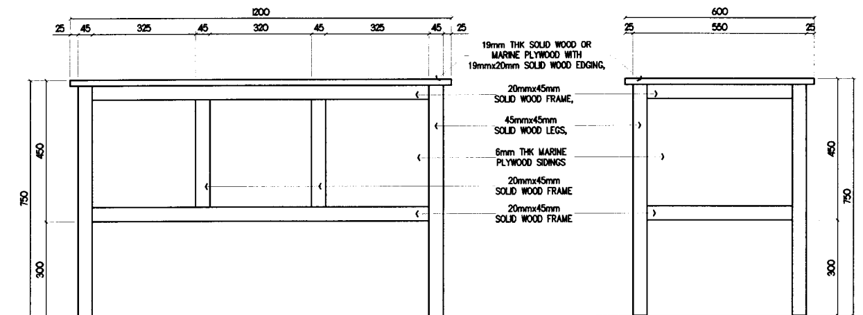
2 FRONT ELEVATION 2 SCALE 1 : 40 M
