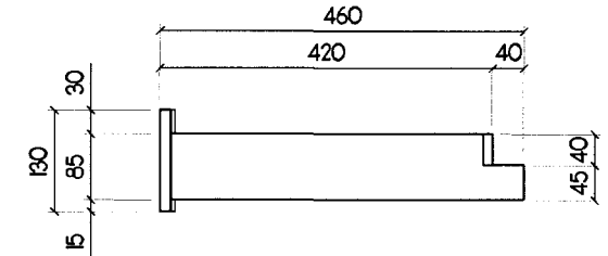
4 RIGHT-SIDE VIEW 8 SCALE 1 : 25 M
