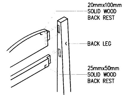
WOOD JOINT- BACK REST 8 SPOT DETAIL- 3 2 SCALE 1:25 M
