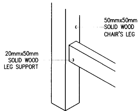
TYPICAL WOOD JOINT 7 SPOT DETAIL- 2 2 SCALE 1:25 M
