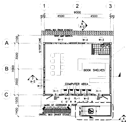
3 SCHOOL LIBRARY FLOOR PLAN A-2 SCALE 1:100M
