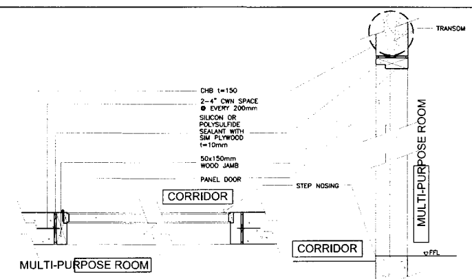
3 DOOR FRAME TYPICAL PLAN & SECTION DETAIL A-5 SCALE 1:5M
