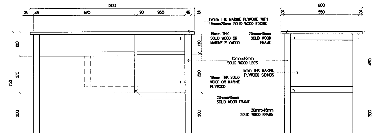
4 REAR ELEVATION 2 SCALE 1 : 40 M
