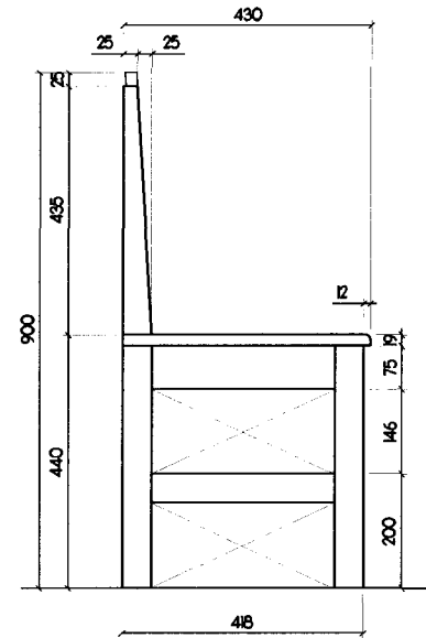
3 LEFT-SIDE VIEW 2 SCALE 1:25 M
