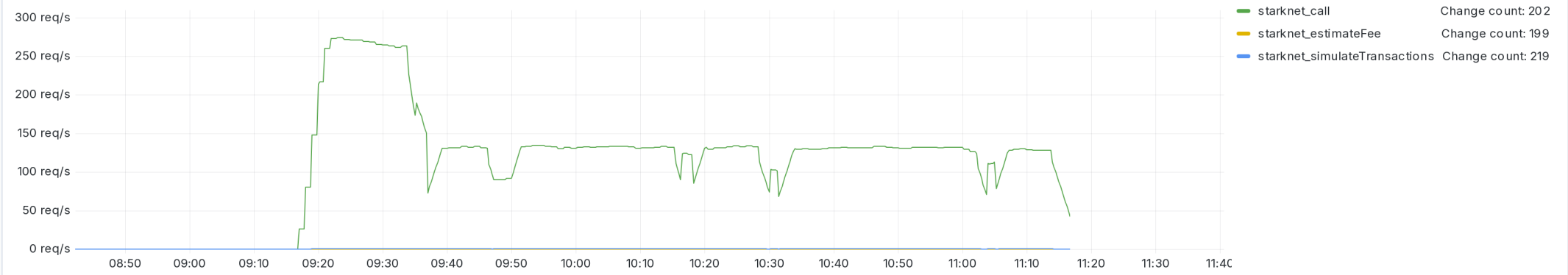
Failed Requests
