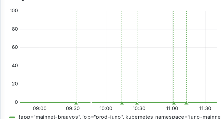
Reorgs
