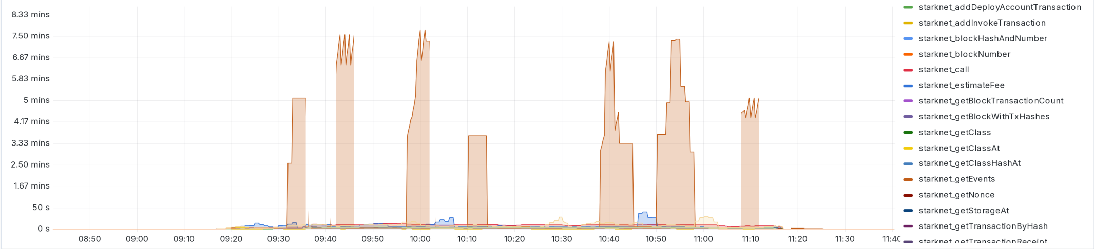
Failed Requests
