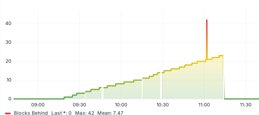
Blocks Behind
