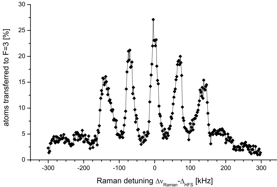
Figure 3.15: Raman spectrum of the vibrational sidebands. Central peak corresponds to the transition on carrier. Peaks to the left and to the right are transitions on red and blue sidebands, respectively.
