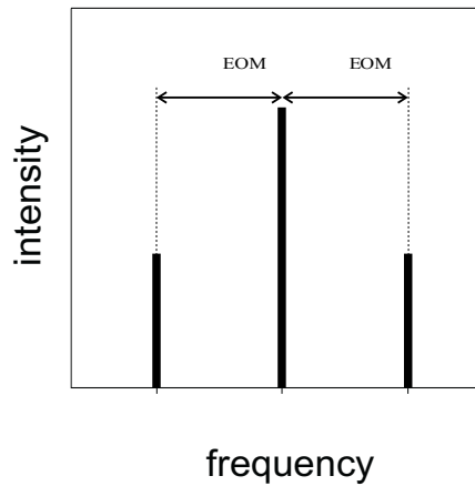
Figure 1.6: Spectrum of our Raman beams
