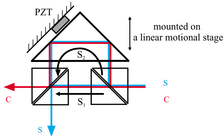
Figure 2.10: Separation of carrier and sidebands using the HDW interferometer.
