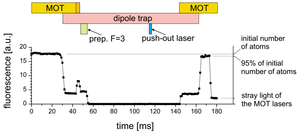
(b) Preparation in F = 3 . About 95 % of atoms are still trapped.
