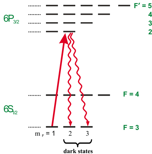
Figure 2.7: Optical pumping into dark m_F states. In the presence of a magnetic field component perpendicular to the quantization axis, the two outermost m_F states become mixed with other m_F states and the total fluorescence increases.
