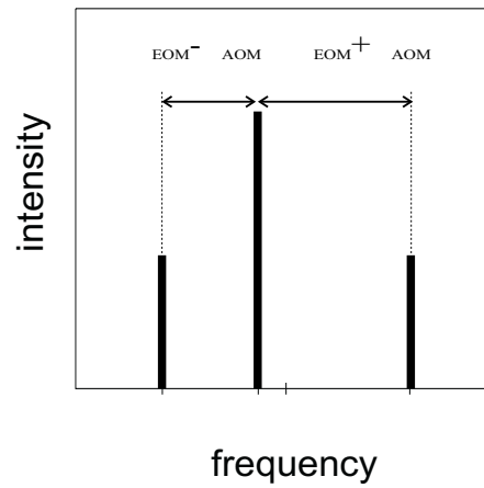
Figure 1.8: Shifted carrier with respect to the sidebands. The EOM frequency must be detuned to \Delta_{\text{EOM}} = \Delta_{\text{HFS}} + \Delta_{\text{AOM}} .
