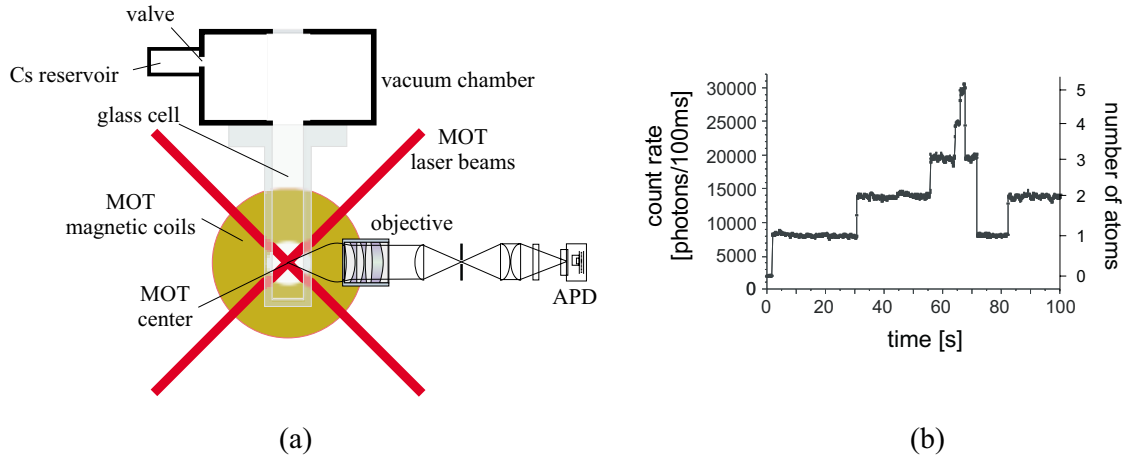
Figure 2.3: (a) The scheme of the vacuum apparatus, the MOT setup and the imaging optics. The third pair of the MOT beams is perpendicular to the image plane. (b) The fluorescence seen by the APD depends on the number of atoms trapped in the MOT. The steps up and down in the fluorescence correspond respectively to the capture and loss of an atom.
