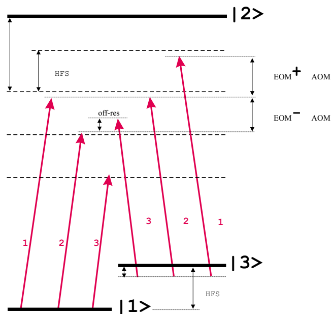
Figure 1.9: Level scheme with one of the Raman transitions suppressed.
