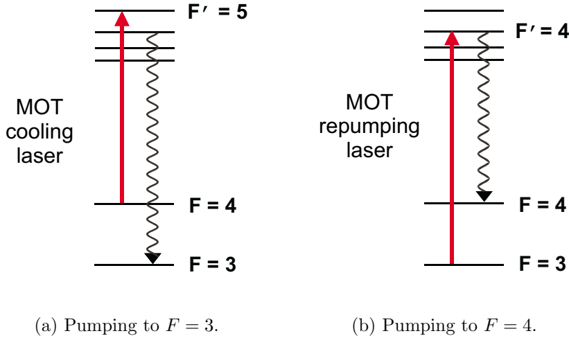
Figure 3.1: Preparation of the initial atomic state. The MOT cooling laser is used for optical pumping to the F = 3 level via the off-resonance excitation of the F' = 4 state. The MOT repumping laser pumps atoms to the F = 4 level.
