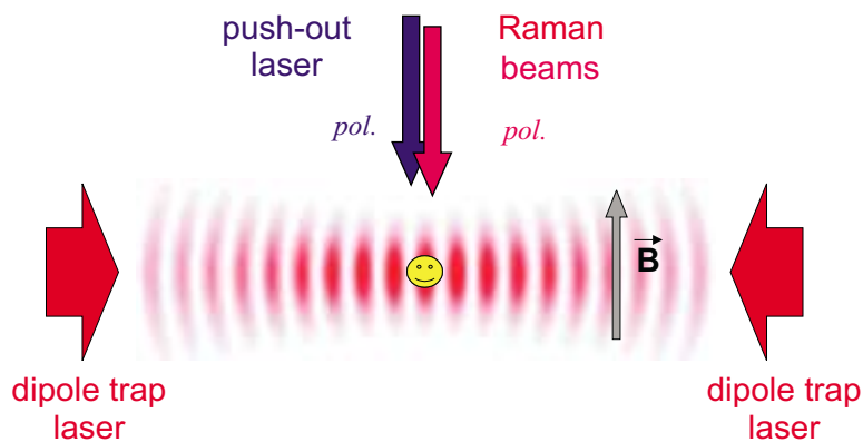
Figure 3.6: Beam geometry for the Raman spectroscopy of Zeeman sublevels.
