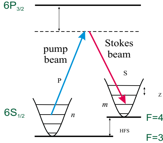
Figure 1.5: Raman transition coupling different vibrational levels.
