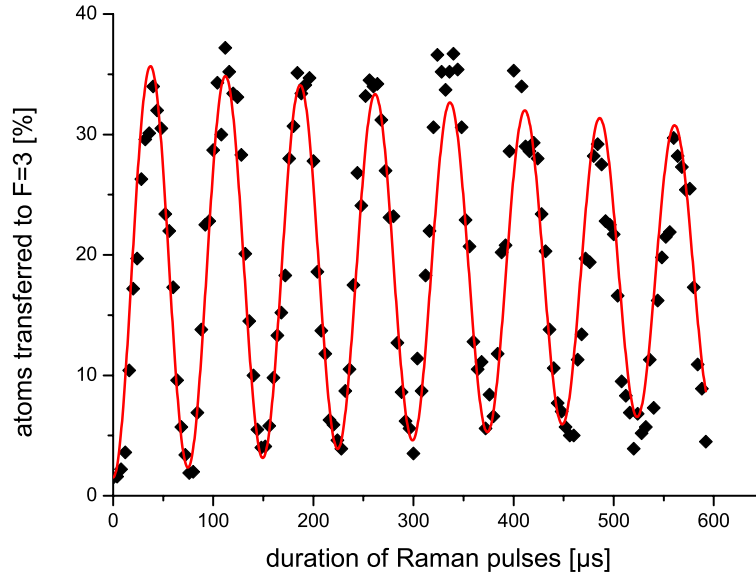
Figure 4.1: Rabi oscillations induced by the Raman lasers.
