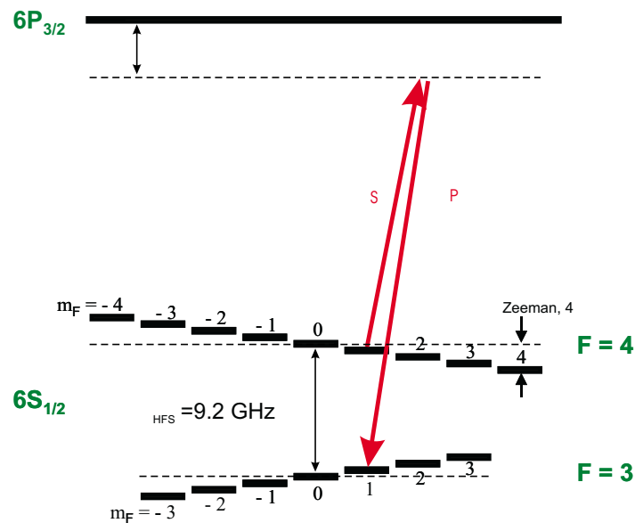
Figure 3.5: Zeeman splitting of the Cs ground states in the presence of a magnetic field.
