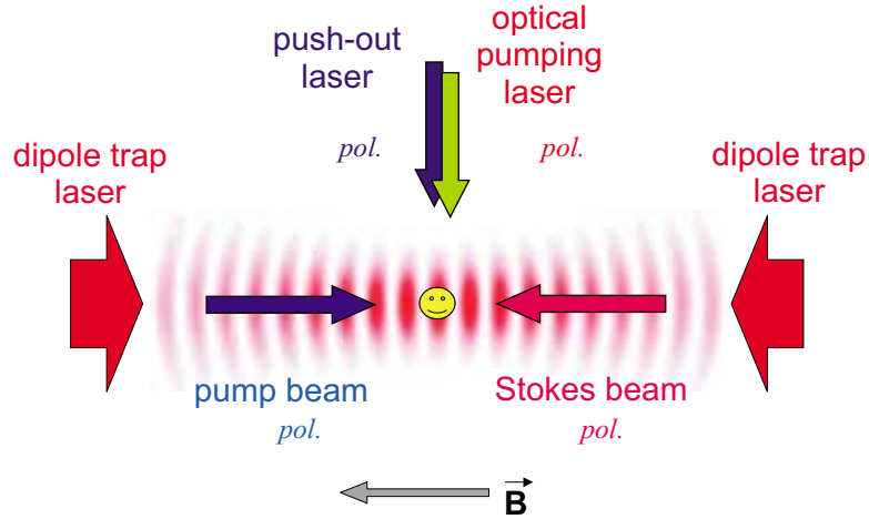
Figure 3.14: Orientation of laser beams and guiding field for Raman spectroscopy of the vibrational sidebands.
