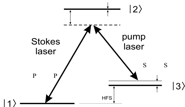
Figure 1.1: Three-level atom coupled by two lasers in \Lambda -configuration.
