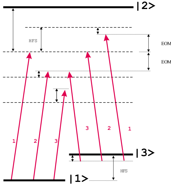
Figure 1.7: Coupling of three Raman lasers with a three-level atom
