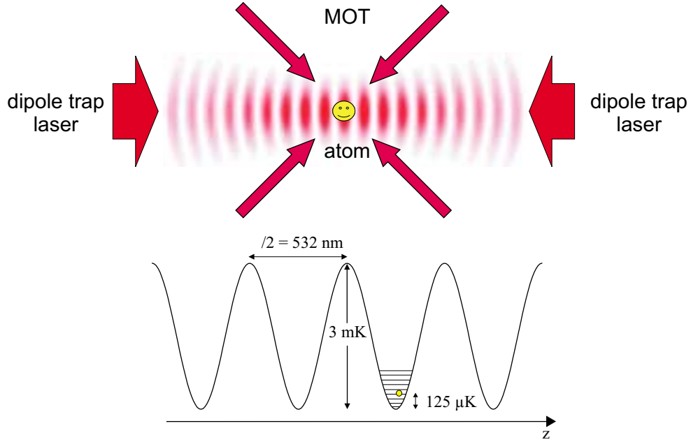
Figure 2.5: An atom trapped in an optical dipole trap formed by the standing wave interference pattern.
