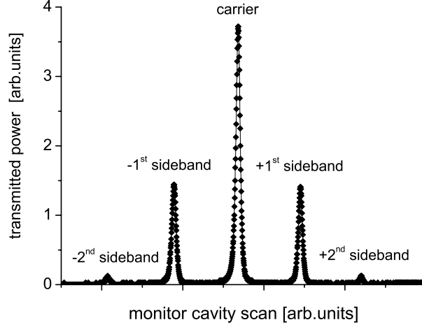
Figure 2.9: Carrier frequency and sidebands generated by the EOM as seen behind a scanning monitor cavity. The fraction of power in the carrier and the 1 st sidebands are about 51 % and 21 % respectively.
