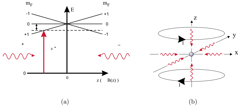
Figure 2.1: Principle of operation of a magneto-optical trap. (a) Simplified atomic level scheme in a one-dimension gradient field interacting with two red-detuned laser beams. (b) A three-dimensional MOT.
