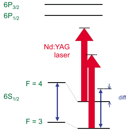
Figure 2.6: Scheme of the differential light shift of the Cs ground levels produced by Nd:YAG laser (greatly exaggerated).
