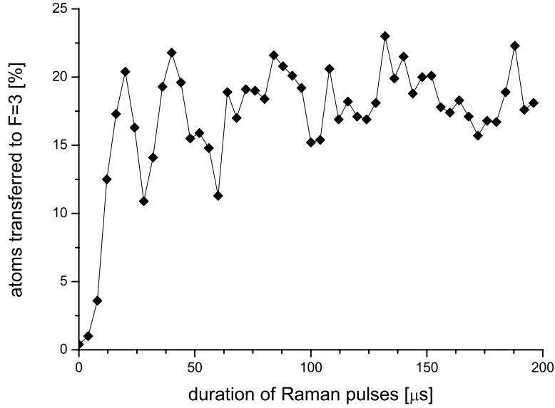
Figure 4.2: Rabi oscillation in the presence of interfering Raman transitions with fluctuating relative phases.
