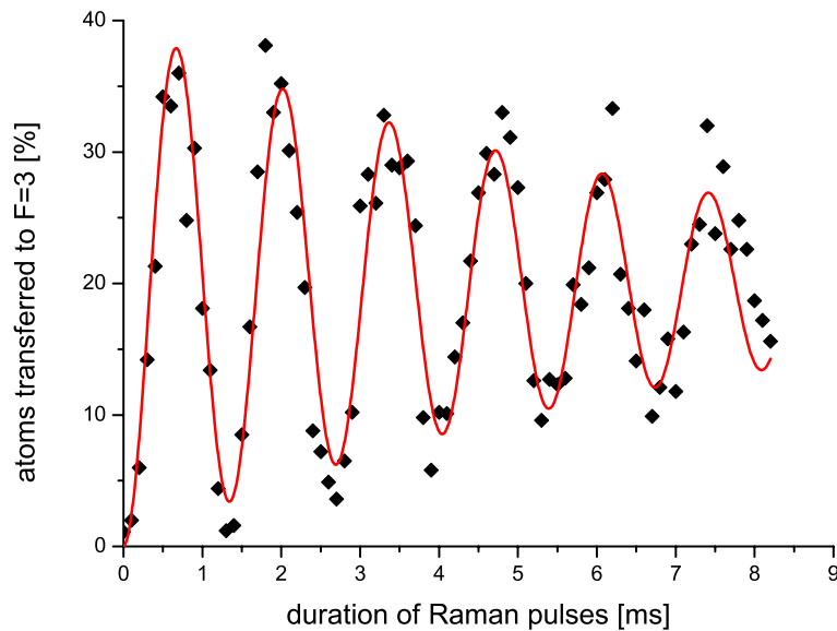
Figure 4.3: Rabi oscillations in the presence of the interference of two Raman transitions.
