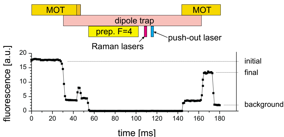
Figure 3.4: Experimental sequence for a Raman spectroscopy experiment. The only information obtained is the initial, final and background fluorescence levels. The fluorescence is accumulated over 10 repetitions.
