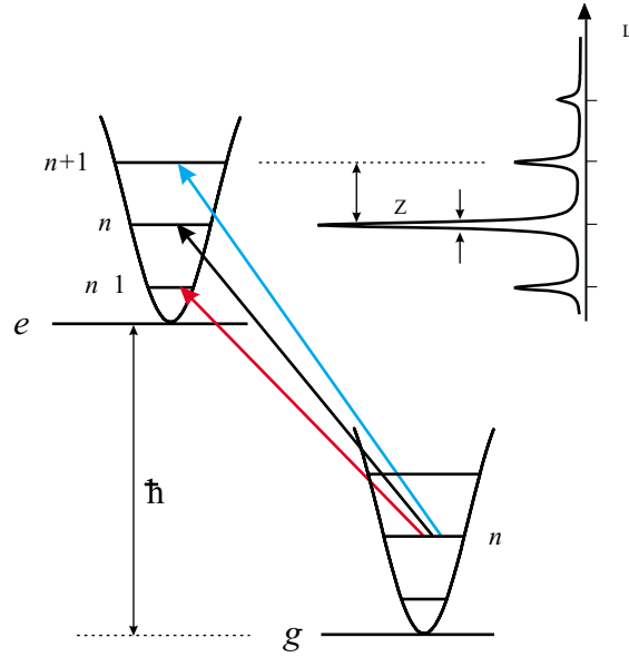
Figure 1.4: Two-level atom in a harmonic potential. Transitions to different vibrational levels result in the appearance of sidebands in the absorption spectrum. The sidebands can be resolved only if the transition linewidth is much smaller than the oscillation frequency, \Gamma \ll \Omega_z .
