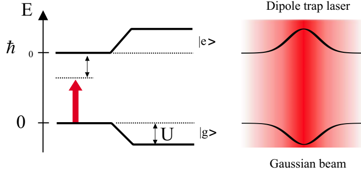
Figure 2.4: Ac Stark effect. A red-detuned laser coupled to a two level atom shifts an atomic ground level downwards. A beam with a Gaussian profile produces a potential well where the atom can be trapped.
