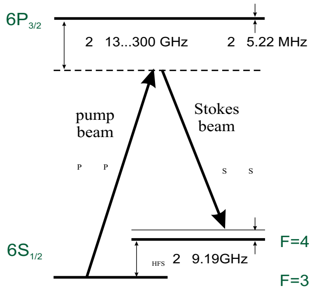
Figure 1.2: Two-photon Raman stimulated transition connecting two Cs hyperfine ground states.
