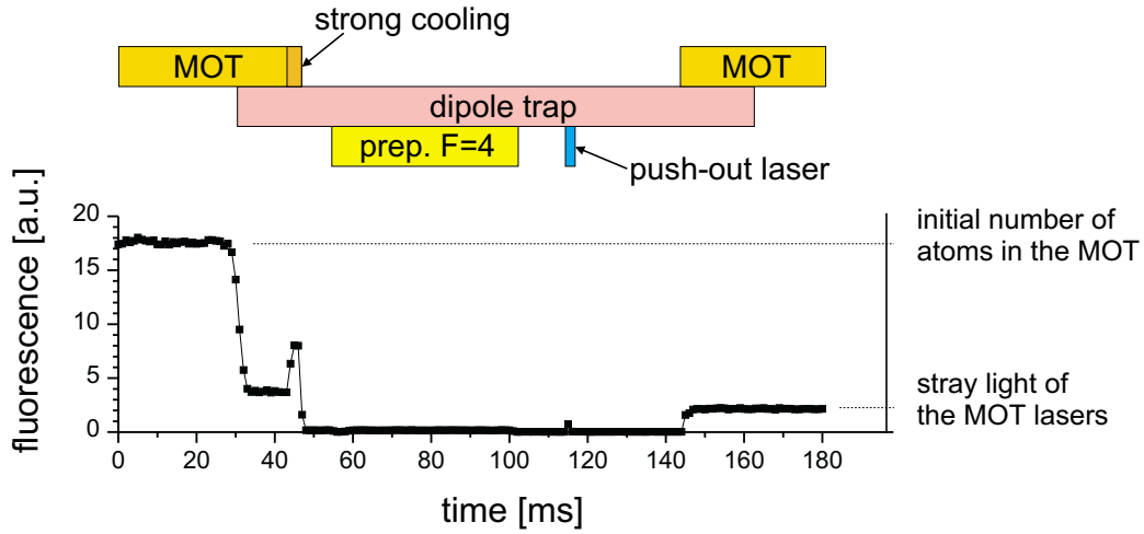
(a) Preparation in F = 4 . No atoms survive after the pushing-out.
