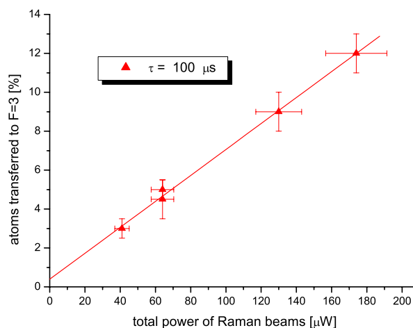
Figure 3.10: Dependence of the off-resonant population transfer of atoms on the total intensity of the Raman beams.
