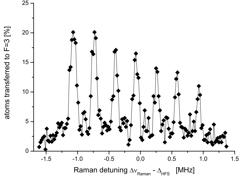
Figure 3.7: The measured Raman spectrum of the Zeeman sublevels.
