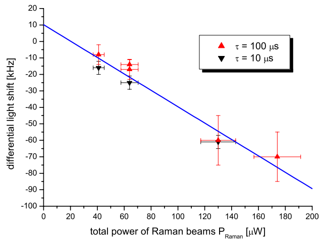
Figure 3.12: Differential light shift of the (F = 4, m_F = 0) \rightarrow (F = 3, m_F = 0) transition.
