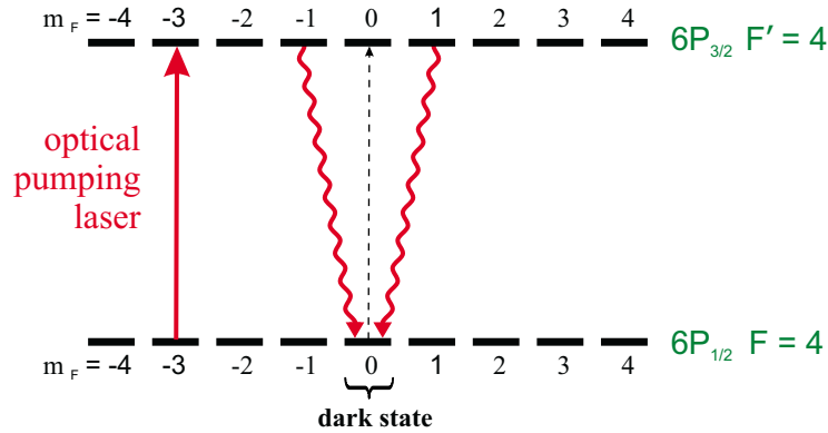
Figure 3.13: Optical pumping into the m_F = 0 state.
