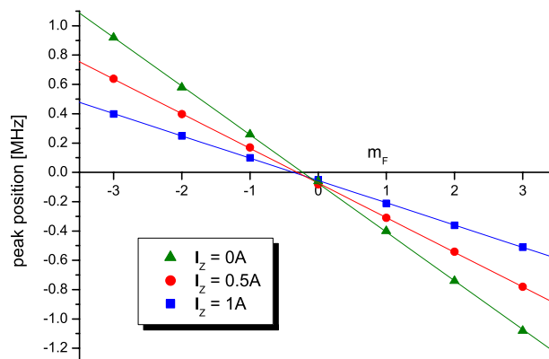
Figure 3.8: Zeeman splitting of m_F sublevels for different values of the current in the z magnetic coils.
