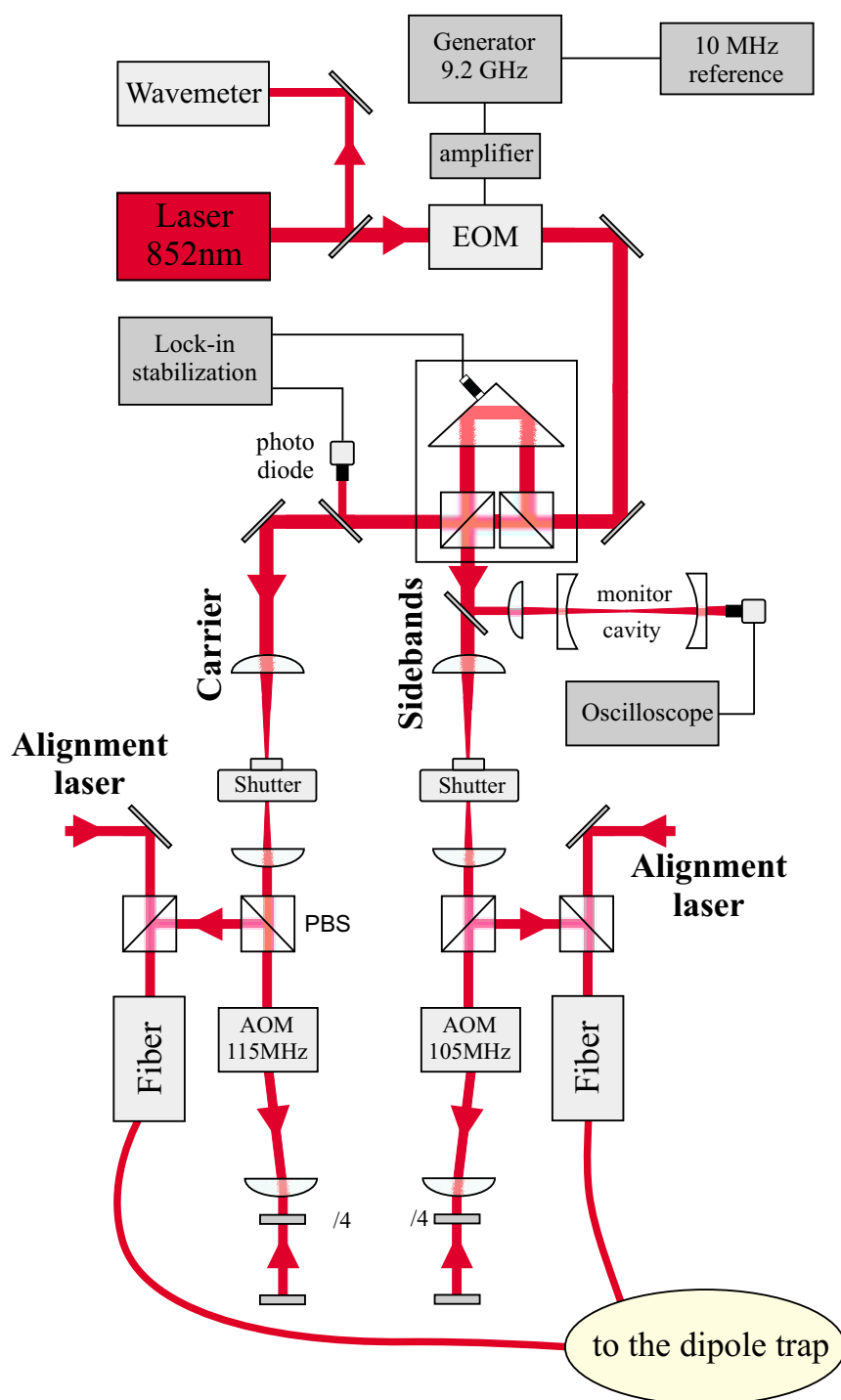
Figure 2.8: Scheme of generation of the Raman beams.
