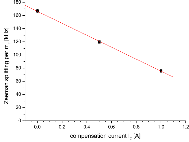
Figure 3.9: Dependence of the Zeeman splitting on the compensation current of the z coil.
