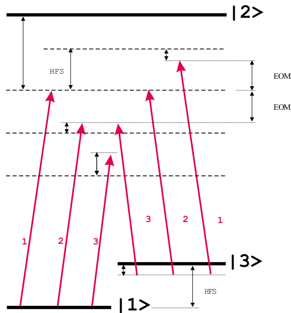
Figure A.1: Coupling of three Raman lasers with a three-level atom
