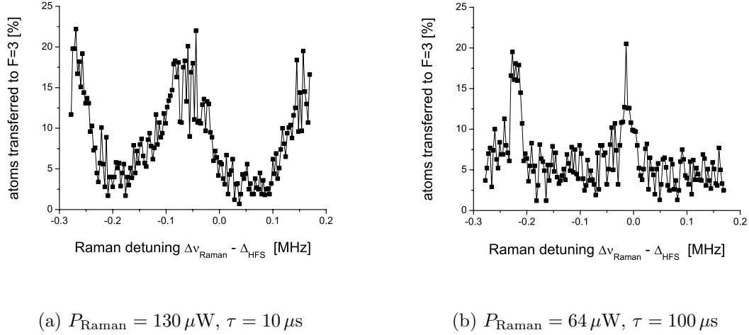
Figure 3.11: Central peak in the Zeeman spectrum, which corresponds to the (F = 4, m_F = 0) \rightarrow (F = 3, m_F = 0) transition, recorded for different pulse durations.
