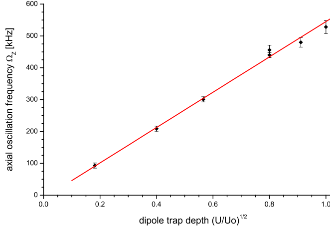
Figure 3.16: Dependence of the oscillation frequency on the dipole trap depth. U_0 denotes the maximal potential depth.
