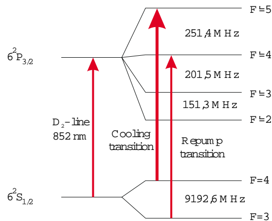
Figure 2.2: Level scheme of the hyperfine structure of the Cesium D_2 -transition.
