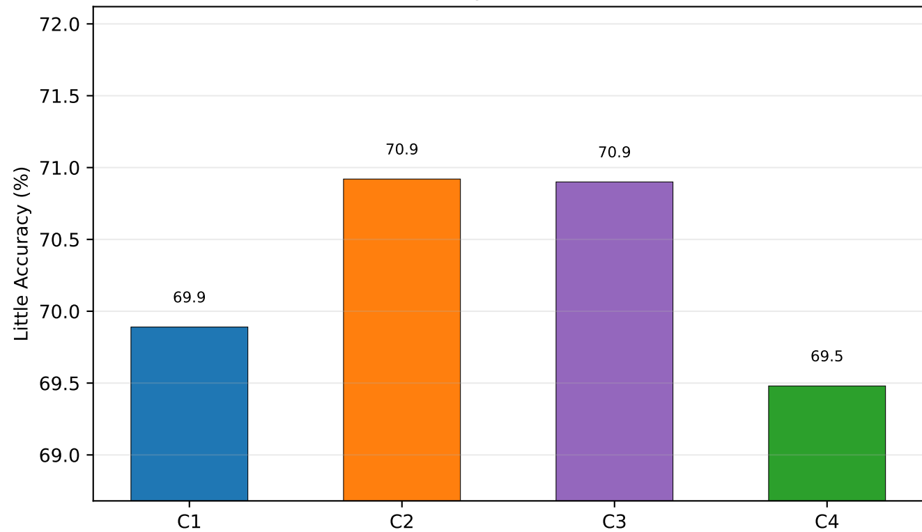
Ablation Little-model Accuracy at Threshold 0.70 - Architecture 2
