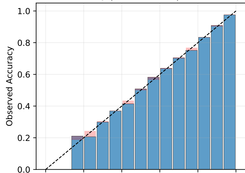
C1: CE only | ECE=0.007 | n=30,000
