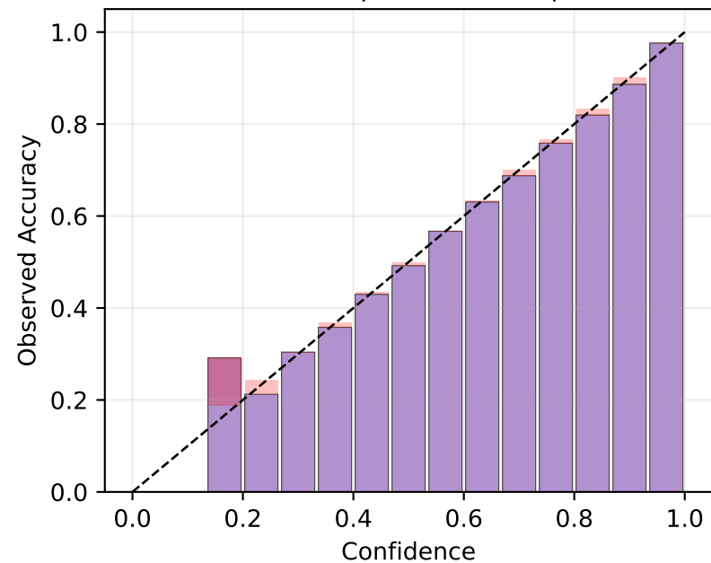
C3: Cascade loss | ECE=0.007 | n=30,000
