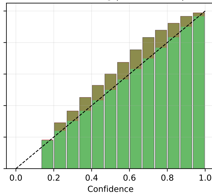
C4: Cascade + smoothing | ECE=0.085 | n=30,000
