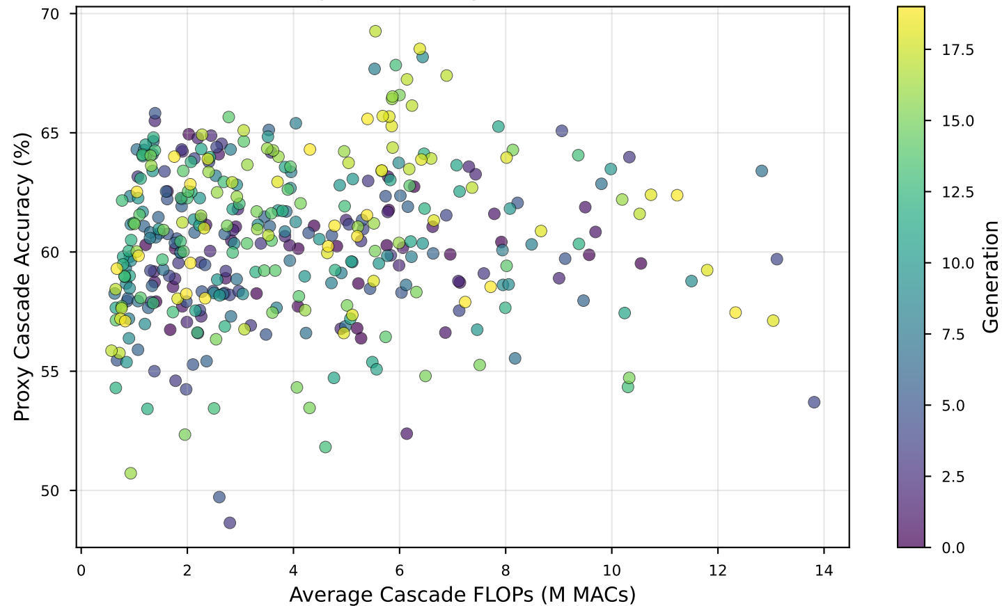
NAS Search Progress (memory hard constraint = 450 KB)
