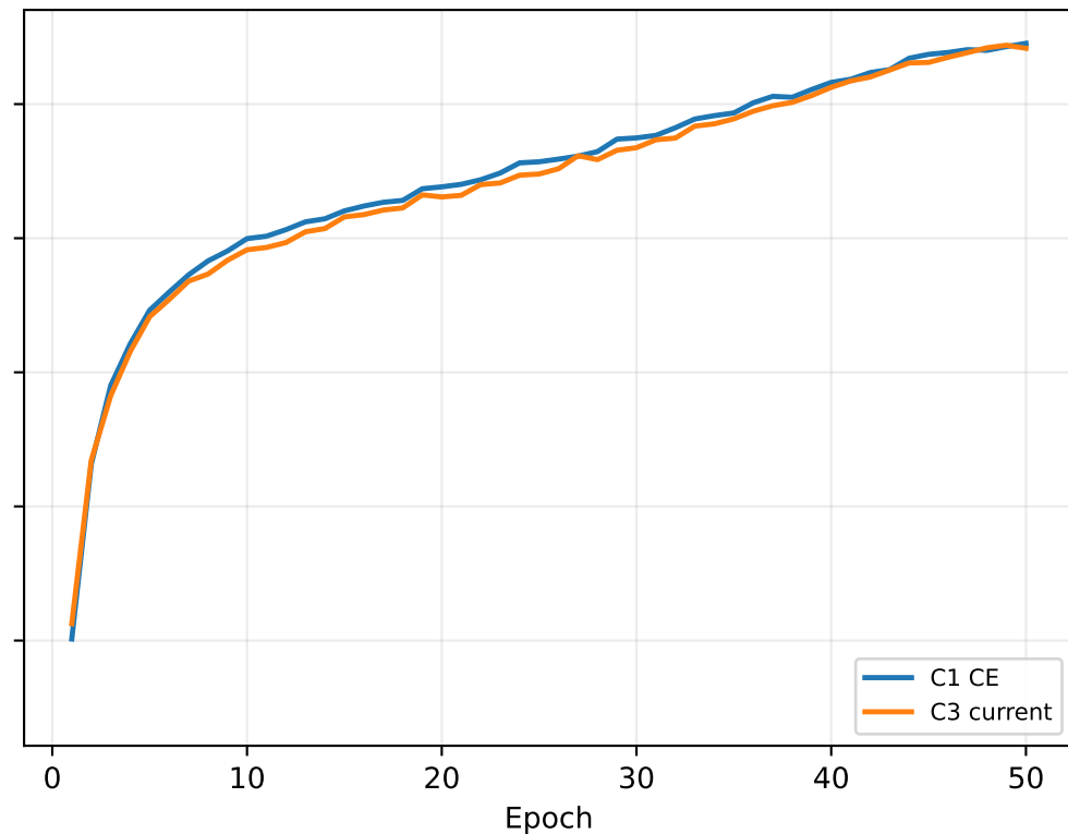
Big Model
