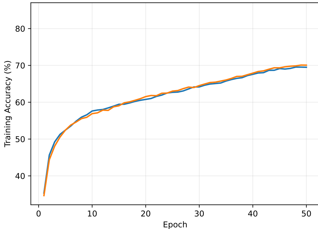
Little Model
