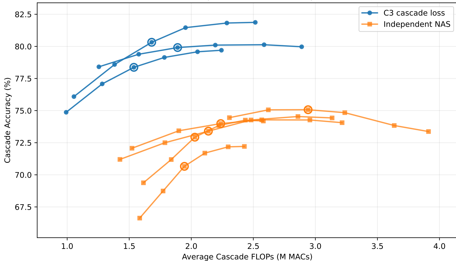
C3 Cascade Loss vs Independent NAS: Accuracy vs Cascade FLOPs
