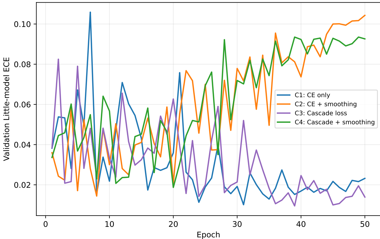
C1-C4 ECE Training Curve Overlay - Architecture 1
