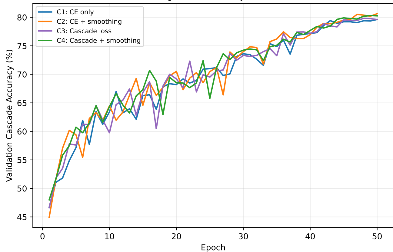
C1-C4 Training Curve Overlay - Architecture 1
