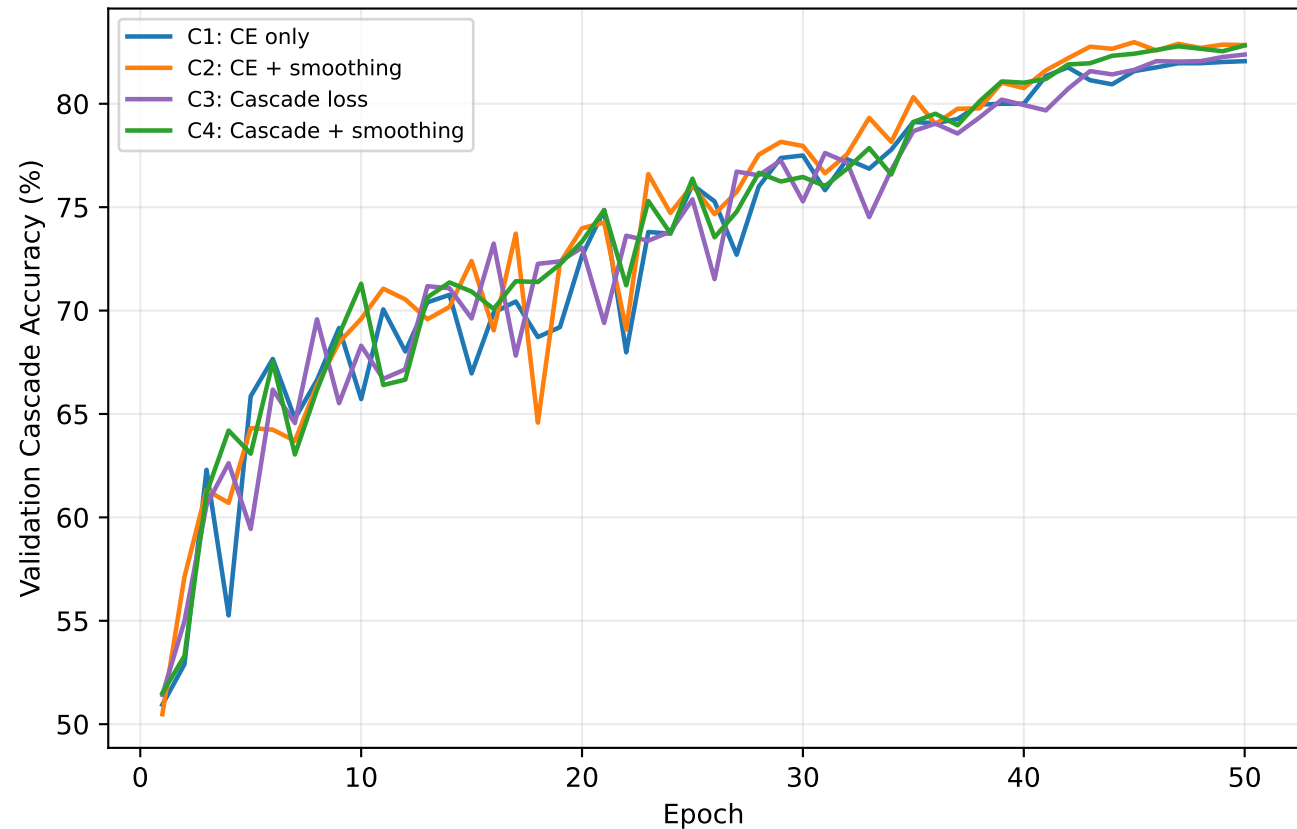
C1-C4 Training Curve Overlay - Architecture 2
