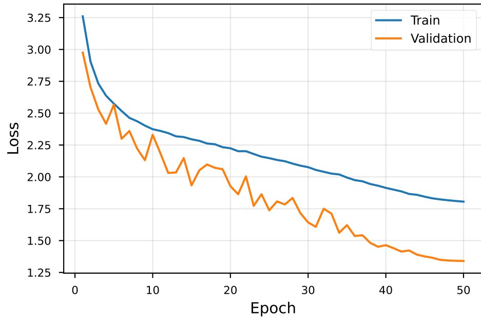
NAS Arch 3 - Loss
