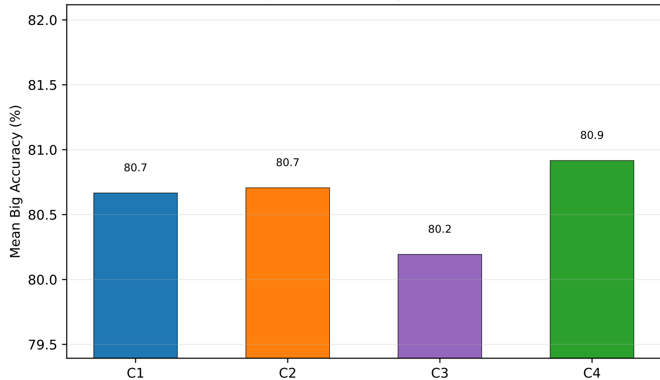
Ablation Big-model Accuracy at Threshold 0.70
