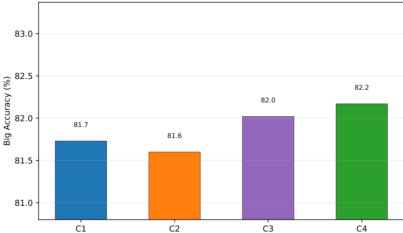
Ablation Big-model Accuracy at Threshold 0.70 - Architecture 2
