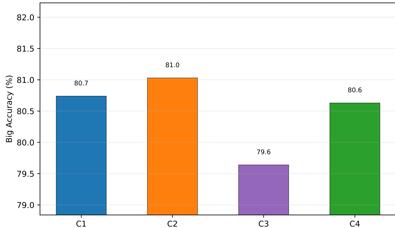
Ablation Big-model Accuracy at Threshold 0.70 - Architecture 3
