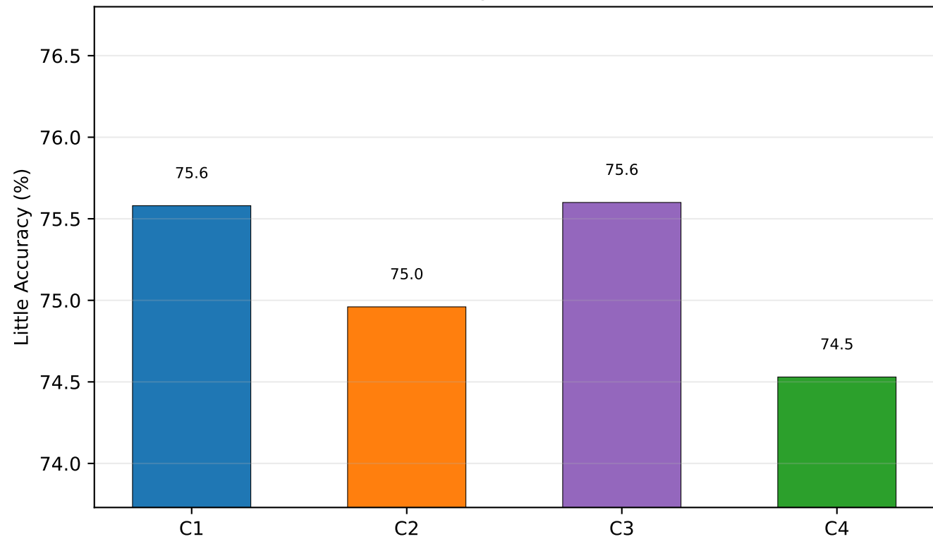
Ablation Little-model Accuracy at Threshold 0.70 - Architecture 3
