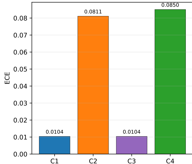
Little-model ECE at Threshold 0.70
