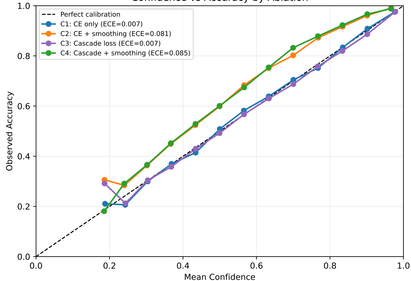
Confidence vs Accuracy by Ablation
